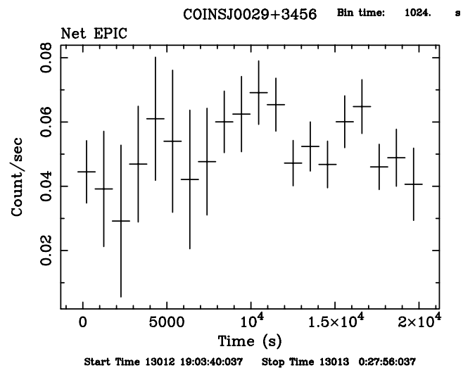
Fig. 1. 0.5–10 keV EPIC (pn and MOS) light curve during the XMM-Newton observation of COINS J0029+3456. The binning time is \Delta t = 1024 \text{ s} . Times are in seconds after the observation start.
