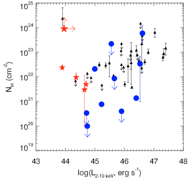
Fig. 8. N_H versus X-ray luminosity for GPS galaxies (stars) and GPS/CSS quasars (filled circles). The small triangles represent the radio-loud quasars observed by ASCA after Reeves & Turner (2000).
