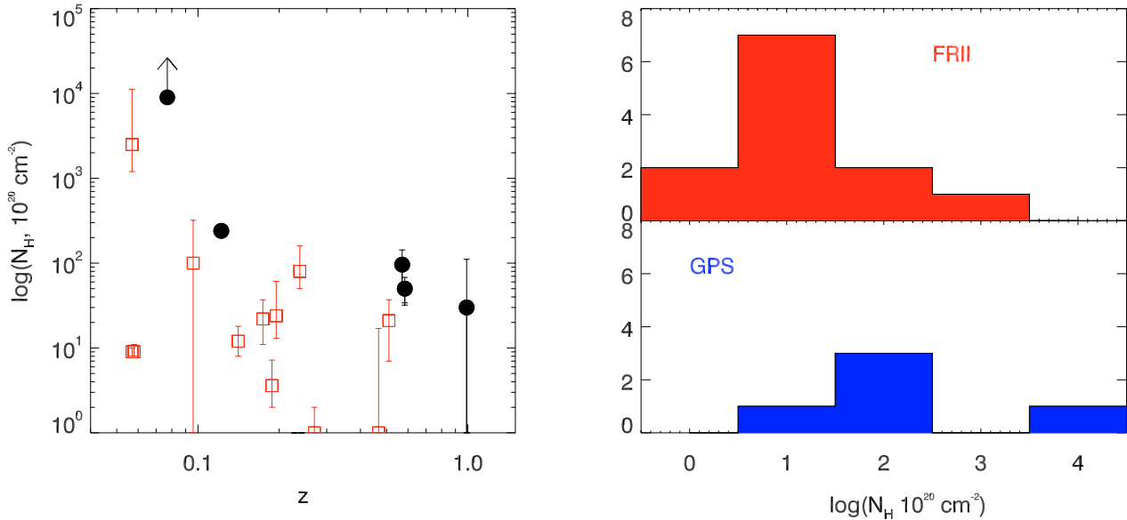
Fig. 6. Left panel: N_{\text{H}} versus z distributions for GPS galaxies (filled circles) and the control sample of FR II radio galaxies (empty squares). Right panel: the N_{\text{H}} distribution functions for FR II radio galaxies (top) and GPS galaxies.
