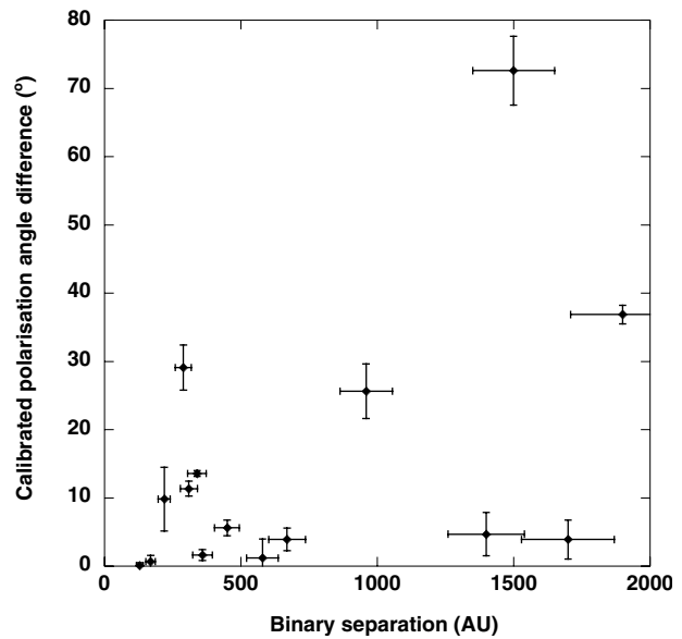
Fig. 11. Discs orientation difference versus separation in AU. The error bars on the position angles are determined in our data reduction pipeline; we plot a 10% error on the distance determination.
