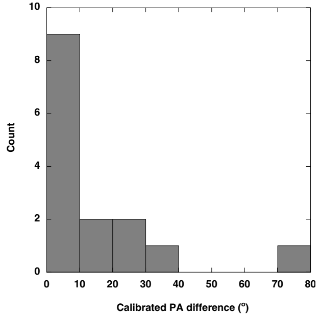
Fig. 10. Histogram of the calibrated position angle difference in the 15 remaining binaries.
