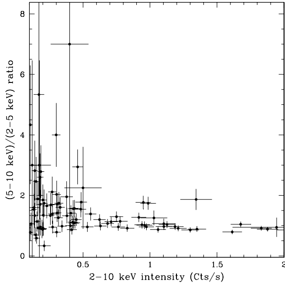
Fig. 2. Hardness-intensity diagram for the 2–10 keV emission of 4U 0114+65 during the BeppoSAX pointing. Although an hint of an inverse correlation between the 5–10 keV/2–5 keV hardness ratio and the 2–10 keV intensity is suggested by the plot, no statistically significant trend is present. Error bars show 1\sigma confidence level uncertainties for each data point.
