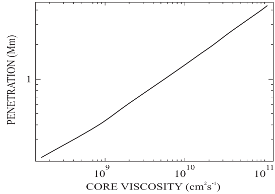
Fig. 3. Penetration depth D_{\text{pen}} of the meridional flow into the radiative interior at latitude 45^\circ in dependence on the viscosity \nu_{\text{in}} prescribed for the radiation interior. The penetration depth runs with \nu_{\text{in}}^{0.5} .
