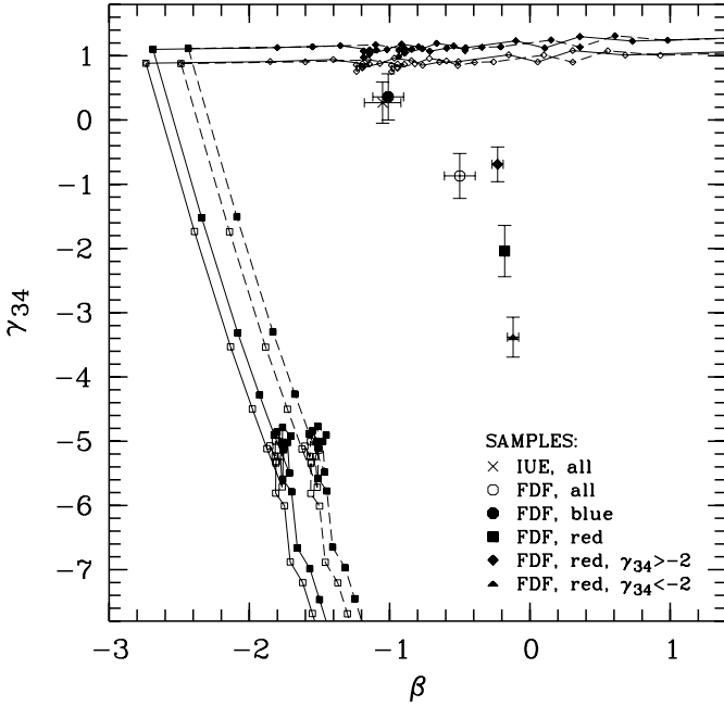
Fig. 10. The UV-bump indicator \gamma_{34} as a function of the reddening measure \beta for our local galaxy sample (cross) and different subsamples of 2 < z < 2.5 FDF galaxies. The complete FDF sample of 34 galaxies (open circle) was divided into a blue ( \beta < -0.4 ; 16 objects; filled circle) and a red subsample ( -0.4 < \beta < 0.1 ; 16 objects; filled square) excluding two very red objects with \beta \sim 1 . Moreover, the red sample was further fragmented into two subsamples of eight objects each differing in \gamma_{34} . The filled lozenge and the filled triangle mark galaxies with \gamma_{34} > -2 and \gamma_{34} < -2 , respectively. The 1\sigma error bars indicate mean errors. The diagram also shows combined stellar population synthesis and radiative transfer models as a function of the optical depth of the dust. Details of the models shown are indicated in the legend of Fig. 9a.
