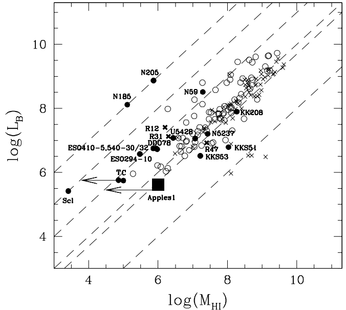
Fig. 2. Filled black square: APPLES 1. Open circles: Local Group (Mateo 1998), Cen A, Sculptor, M 81, M 83, IC 342, Maffei, Canes Venatici I groups (Huchtmeier et al. 2000; Karachentsev et al. 2001; Paturel et al. 2003; Karachentsev 2005; Bouchard et al. 2005). Crosses: field dwarf galaxies (van Zee 2001; Roberts et al. 2004). All dSphs/transition-type dwarfs are represented with filled or bold symbols and labelled with their names (to avoid confusion the names of the dSphs field galaxies taken from Roberts et al. 2004 are shortened using an “R” followed by the number of the source reported in their Table 1). The dashed lines correspond to a constant M_{\text{HI}}/L_B ratio of 100, 2, 1, 0.1, 0.01, and 0.001 from right to left.
