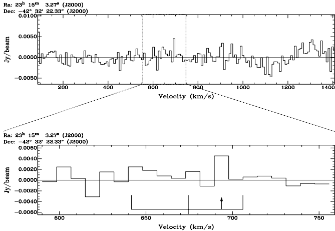
Fig. 1. Full velocity range ( upper panel ) and close-up ( lower panel ) HI Parkes spectrum of APPLES 1, which has been smoothed by a factor of ten. The velocity resolution is 8.3 \text{ km s}^{-1} and the rms ( 1\sigma ) per channel is 1.74 \text{ mJy/beam} . The beam ( HPBW ) is \sim 14' . The thick lines in the lower panel indicates the recession velocity of the galaxy together with its uncertainty, V_{\text{hel}} = (674 \pm 30) \text{ km s}^{-1} . The arrow marks the weak feature possibly due to HI emission from APPLES 1.
