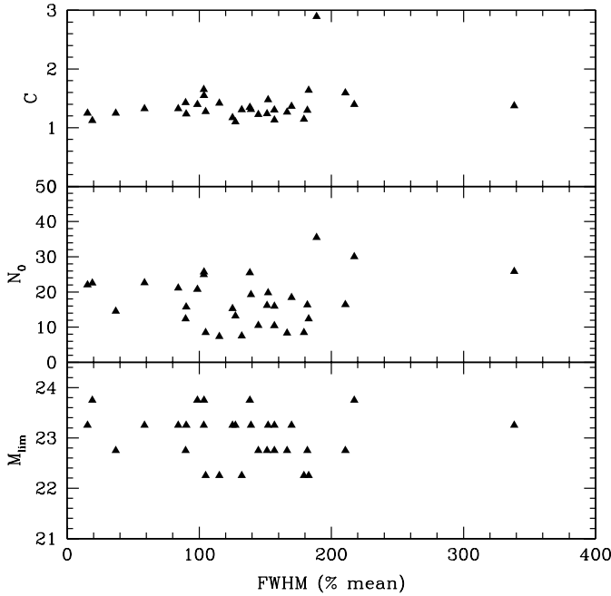
Fig. 7. The dependence of limiting magnitude ( M_{\text{lim}} ), normalisation ( N_0 , in galaxies per square arcmin) and slope ( C ) on structure in the foreground disk. Structure is characterized by the FWHM of the distribution of mean pixelvalues of the 100^2 pixel sections. Expressed as a percentage of the mean of that distribution.
