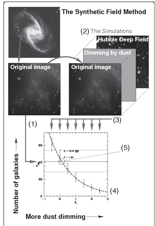
Fig. 1. A schematic of the “Synthetic Field Method”. First a WFPC2 field is retrieved from the Hubble Space Telescope archive and redshifted. The Synthetic Field Method itself consists of the following steps: 1. the number of distant galaxies in the original science field are counted; 2. the “synthetic fields” are made by combining a dimmed Hubble Deep Field with the science field; 3. the numbers of synthetic galaxies are counted in the synthetic fields; 4. Eq. (1) is fitted to the number of synthetic galaxies as a function of the applied dimming; 5. from the intersection between the number galaxies in the science field and the fit, the average dimming in the image is found.
