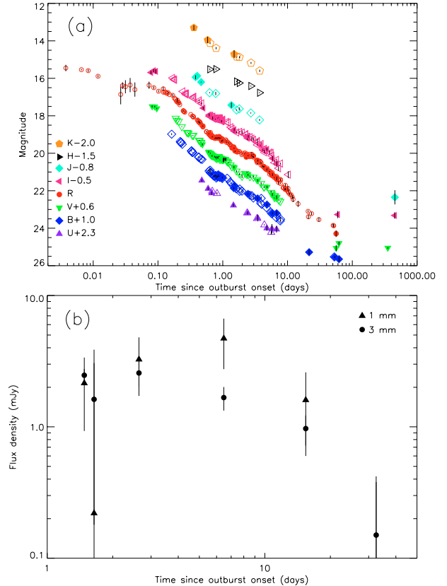
Fig. 2. a) Optical and NIR light curves of GRB 021004 for the first ~500 days after the event. The different bands have been intentionally separated for clarity. Our observations are marked with filled symbols while published data are represented with void ones (see text for references). b) Millimetre light curves for the first ~35 days, obtained at PdB.
