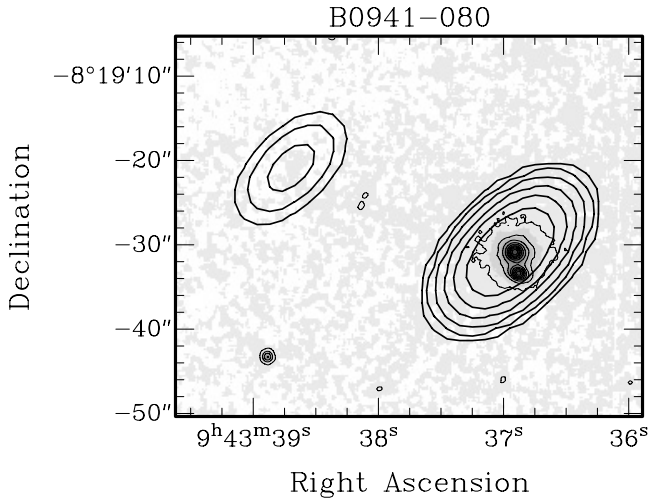
Fig. 7. Radio contours of 0941-080 at 1.36 GHz superimposed to the NOT optical image (gray scale and thinner contours). First radio contour is 0.5 mJy. Peak in the radio image is 2.726 Jy.
