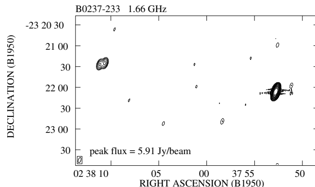
Fig. 2. 0237-233 at 1.66 GHz.
