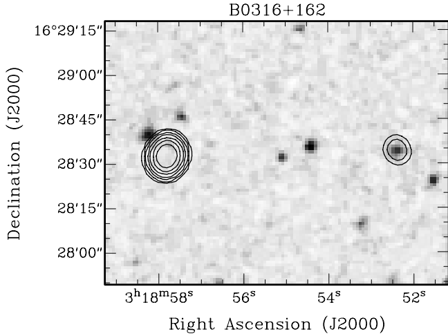
Fig. 4. Radio contours of 0316+162 at 1.36 GHz superimposed to the gray scale POSS2 image.
