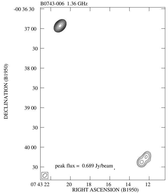
Fig. 6. 0743-006 at 1.36 GHz.
