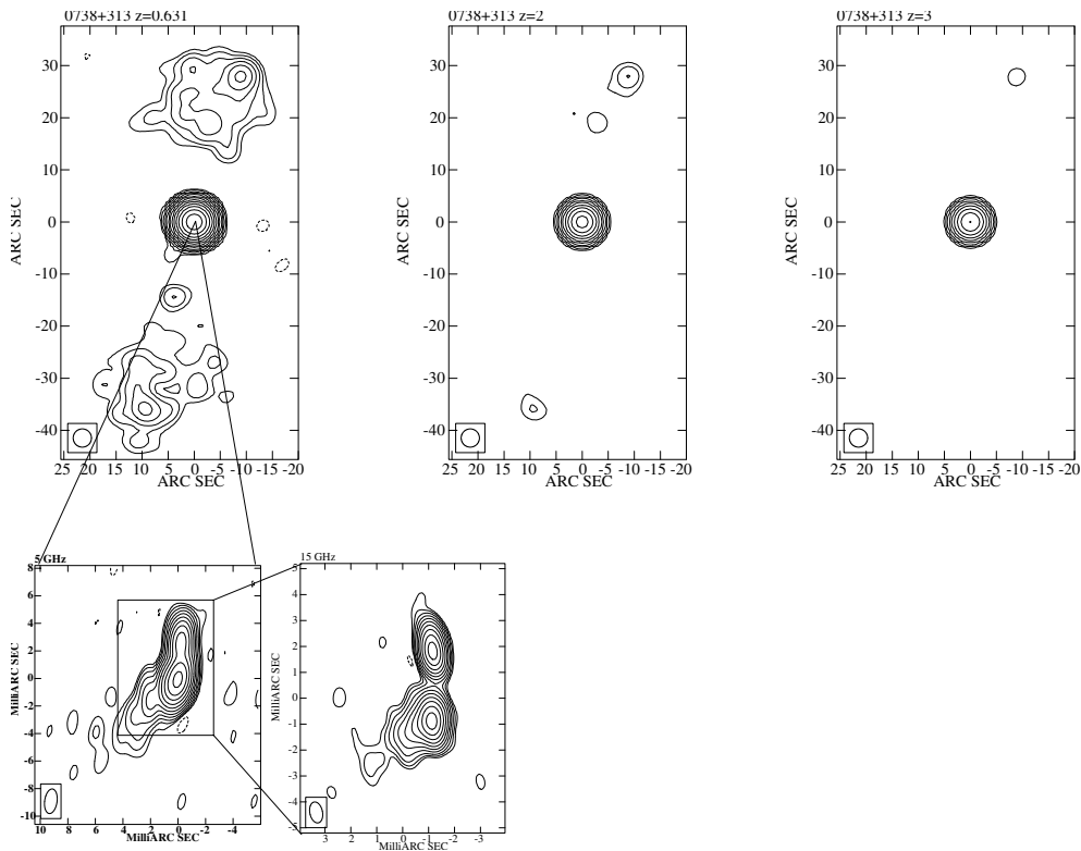
Fig. 17. The effect of redshift on extended emission detectability. Left image is 0738+313 at z = 0.631 , center image is how it would appear at z = 2 , right image is how it would appear at z = 3 . The dependence of angular size with redshift has not been taken into consideration because at these high redshifts angular size does not depend strongly on redshift.
