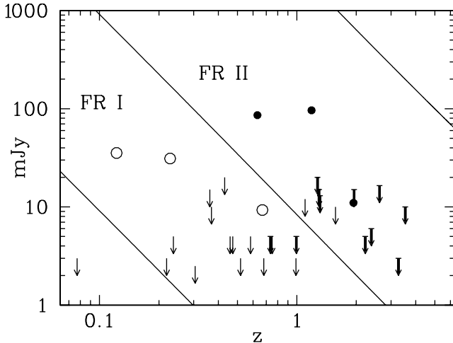
Fig. 18. Flux density at 1.36 GHz of extended emission versus redshift. Continuous lines approximately separate regions of FRI and FR II radio sources, filled circles are quasars, empty circle are galaxies, thick arrows are higher limits for quasars, thin arrows are higher limits for galaxies (see Sect. 4).
