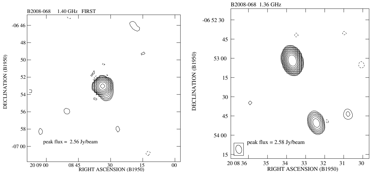
Fig. 14. 2008-068 from the FIRST ( left ) and from present data ( right ).
