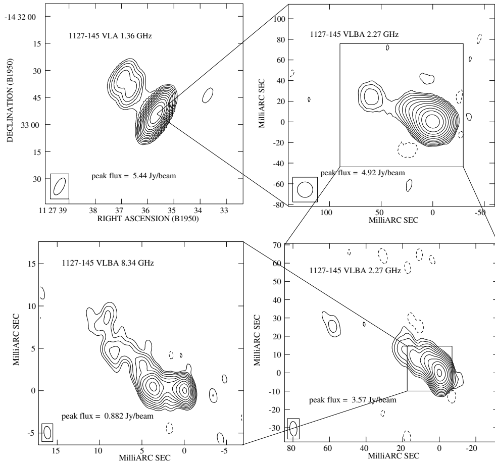
Fig. 9. 1127-145 from mas to arcsecond scale.
