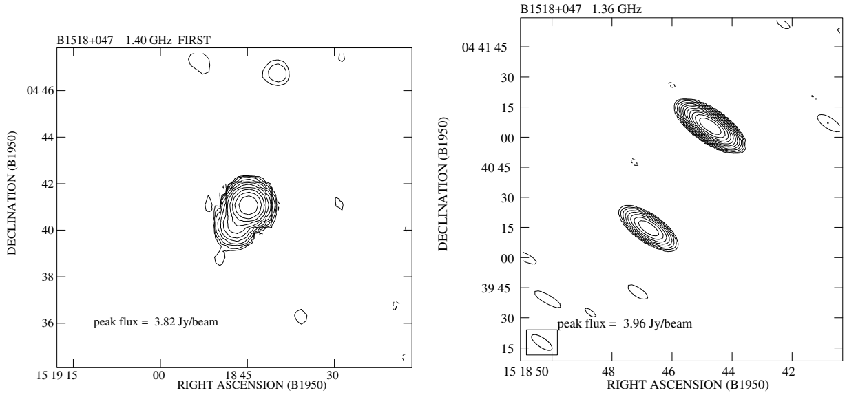
Fig. 13. 1518+047 from the FIRST ( left ) and from present data ( right ).
