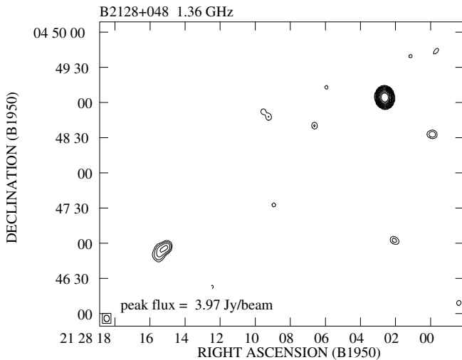
Fig. 15. Radio image of 2128+048 at 1.36 GHz.
