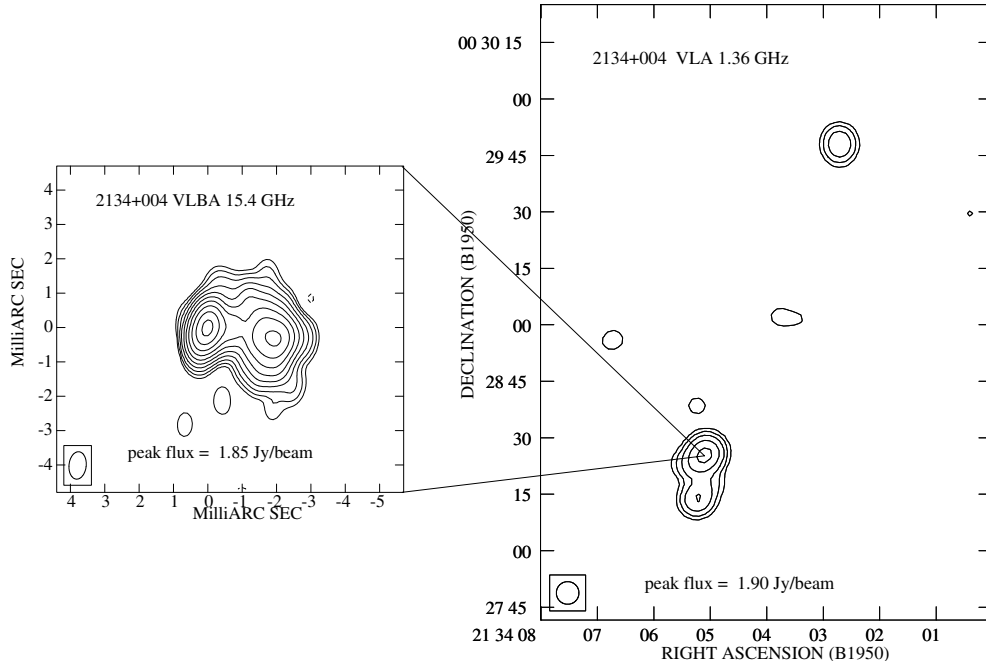
Fig. 16. 2134+004 at mas (left) and arcsecond resolution (right). In the VLA image most of the core flux density has been subtracted to enhance the visibility of the diffuse emission.
