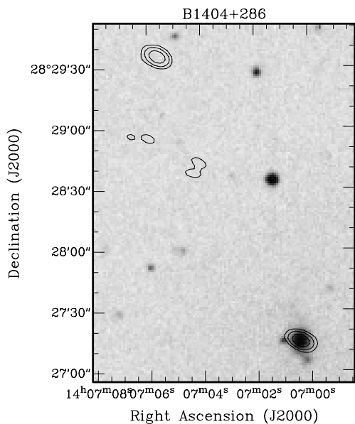
Fig. 12. Radio contours of 1404+286 at 1.36 GHz superimposed to the gray scale POSS2 image
