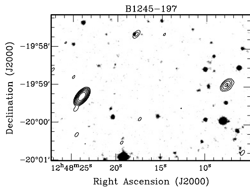
Fig. 10. Radio contours of 1245-197 at 1.36 GHz superimposed to the gray scale POSS2 image.
