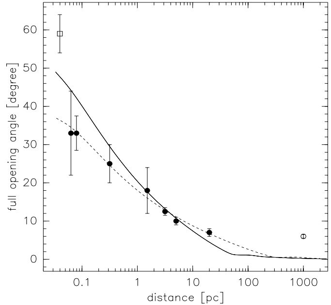
Fig. 2. Comparison of the opening angle calculated from model A and model B, and the observational data for M 87. The black lines represents model A ( solid ) and model B ( dashed ), respectively, while various symbols represent observational measurements. The data points marked by black circles was taken into account in the fitting procedure for model A and B. Model A fits, additionally, the innermost data point ( open square ). The outermost measurement ( open circle ) was disregarded for both models, since it is located beyond knot A (see text).
