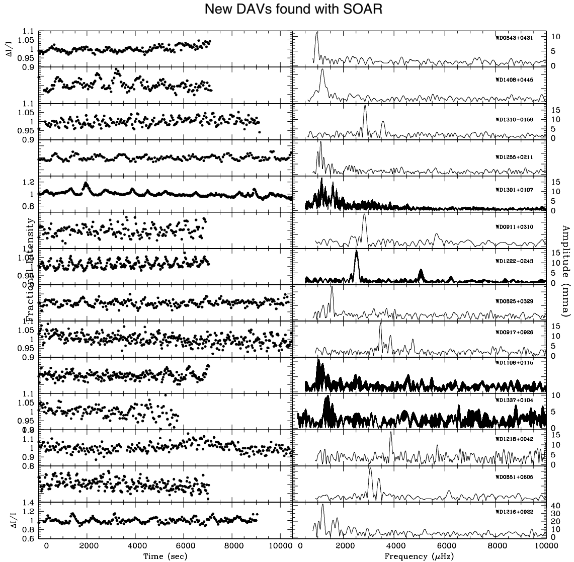
Fig. 1. Light curves ( left panels ) and Fourier transforms ( right panels ) for the new ZZ Ceti. mma is milli-modulation amplitude, corresponding to 1000 \times \Delta F/F , where F is the measured flux.
