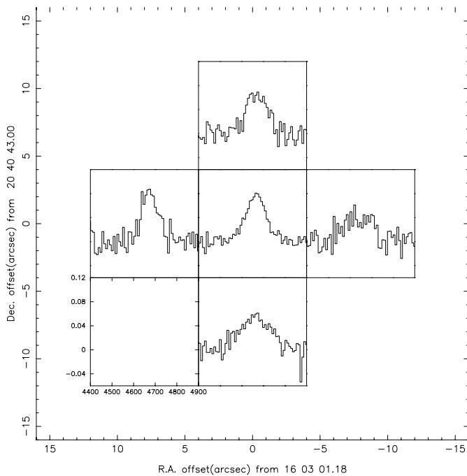
Fig. 3. Grid map of the J = 3-2 CO emission from NGC 6052. Horizontal scale is radial velocity V_{\text{LSR}} in \text{km s}^{-1} , vertical scale is main-beam brightness temperature T_{\text{mb}} in Kelvins.
