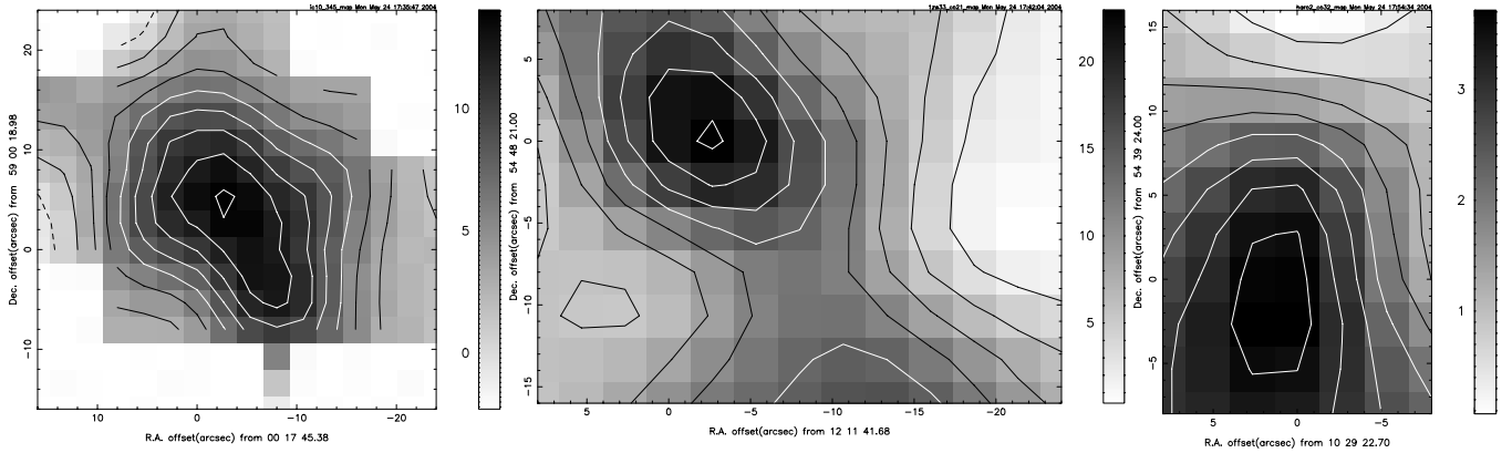
Fig. 2. Contour maps of integrated CO emission. Lowest contour is always at zero. Left: IC 10 ( J = 3-2 ) with main-beam brightness temperature contours in multiples of 1 K. Center: NGC 4194 ( J = 2-1 ) with contours in multiples of 4 K. Right: Haro 2 ( J = 3-2 ) with contours in multiples of 0.75 K.
