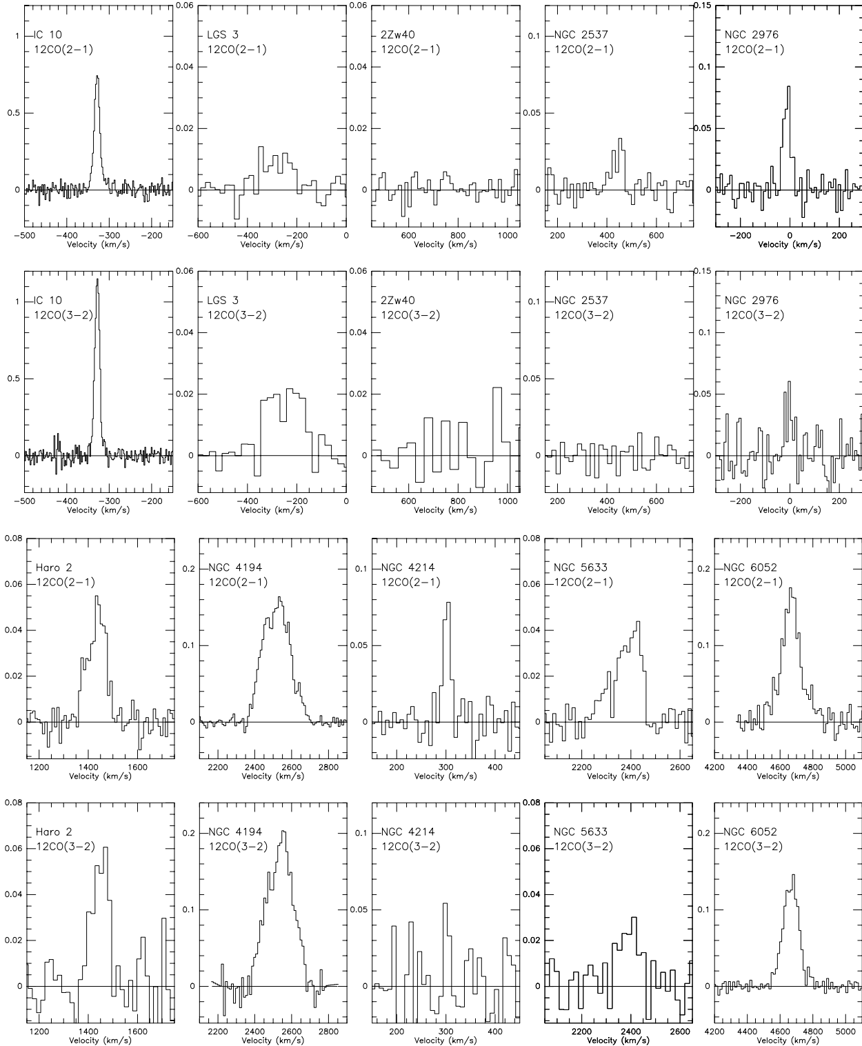
Fig. 1. J = 2-1 and J = 3-2 ^{12}\text{CO} emission-line spectra observed towards the sample dwarf and peculiar galaxies. Horizontal scale is V_{\text{LSR}} in \text{km s}^{-1} , vertical scale is main-beam brightness temperature T_{\text{mb}} in Kelvins.
