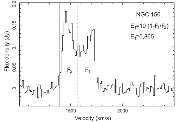
Fig. 5. HI velocity profile of NGC 150, showing the two horns, the center of the profile and the extremity of the two horns. F_1 and F_2 are the integrated flux of each horn, and their ratio gives an estimate of the HI asymmetry.
