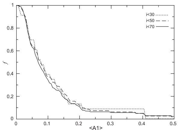
Fig. 3. Cumulative functions of \langle A_1 \rangle (fraction of galaxies with \langle A_1 \rangle larger than the x -axis value) for galaxies seen below a certain cut-off in the inclination angle i ; for i < 30^\circ, 50^\circ , and 70^\circ . The curves are nearly identical, hence the highest value of the cut-off 70^\circ is chosen, as it gives the largest number of galaxies in the sample. Galaxies more inclined than 70^\circ no longer follow the same statistical distribution and have been rejected.
