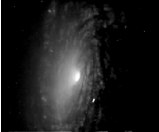
Fig. 2. HST/PC ( F606W ) image of NGC 5033 (FOV: 36'' \times 36'' ), obtained from the data archive at the Space Telescope Science Institute based on observations made with the NASA/ESA Hubble Space Telescope. East is to the left and North is up.
