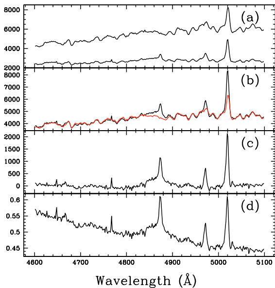
Fig. 5. Comparison between spectra 68 (optical nucleus) and 71 (Seyfert nucleus). a) Original spectra (68 top, 71 bottom). b) Rectified spectra f_{\lambda}^*(68) (red) and f_{\lambda}^*(71) (black). Notice the good agreement among the absorption spectral features except in the region where the H\beta broad emission lies in spectrum 71. c) Difference between the rectified spectra, f_{\lambda}^*(71) - f_{\lambda}^*(68) . d) Quotient between the original spectra, f_{\lambda}(71)/f_{\lambda}(68) .
