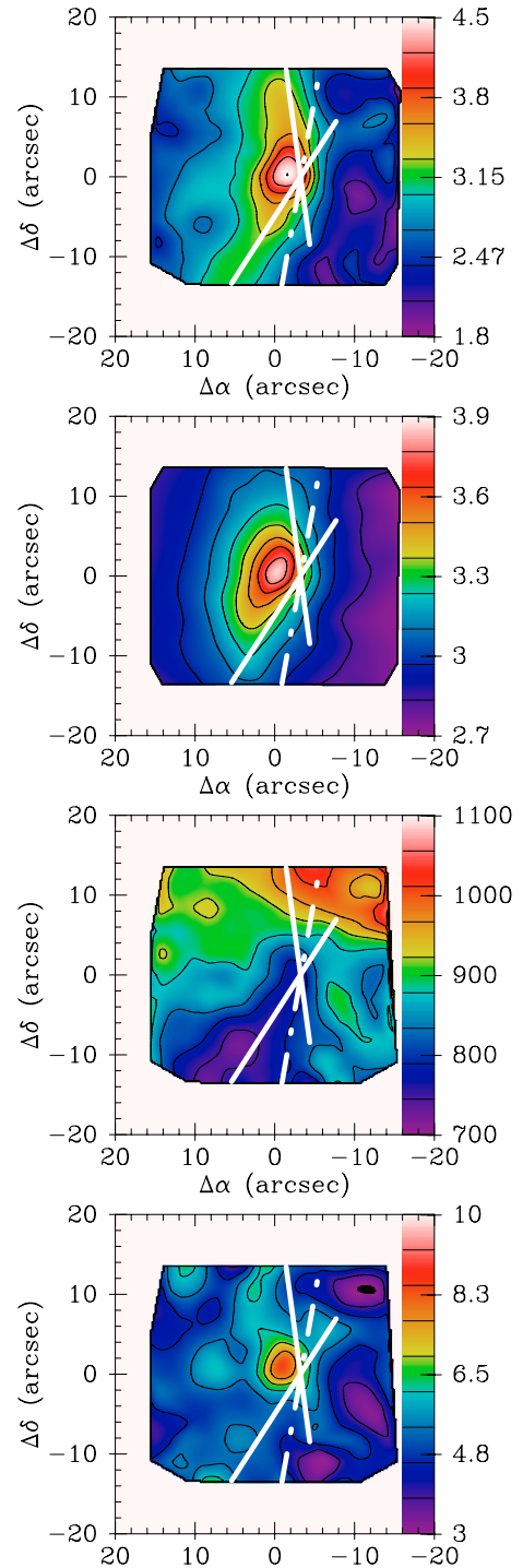
Fig. 7. Tentative ionization cones (white continuous lines) represented on (from top to bottom) the [\text{OIII}] line emission (arbitrary units), the stellar continuum (arbitrary units), the [\text{OIII}] velocity ( \text{km s}^{-1} ), and the [\text{OIII}] FWHM maps ( \text{\AA} ). The dotted dashed line is parallel to the photometric major axis.
