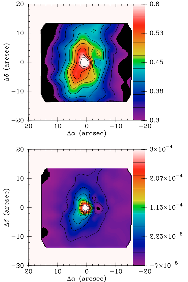
Fig. 3. Top: 5965 Å/4700 Å color map (see text). Bottom: map of SED slopes (see text).
