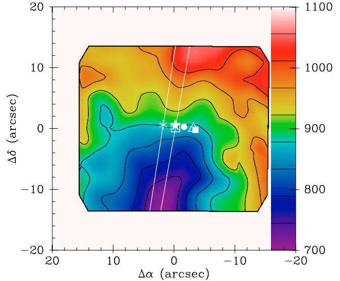
Fig. 6. Photometric and kinematic centers. The eastern white line corresponds to the major axis of the ellipse fitted to the outermost isophote of the stellar continuum in Fig. 1 (apparent photometric major axis). The western white line is the kinematic axis inferred from a ring model fitting to the stellar velocity field. From left to right (east to west) the asterisk, star, square, circle, triangle and filled square represent the center of the ellipse fitted to the outermost continuum isophote, the stellar continuum emission peak, the kinematic center, the [OIII] emission peak, the BLR location and the H\beta emission peak, respectively.
