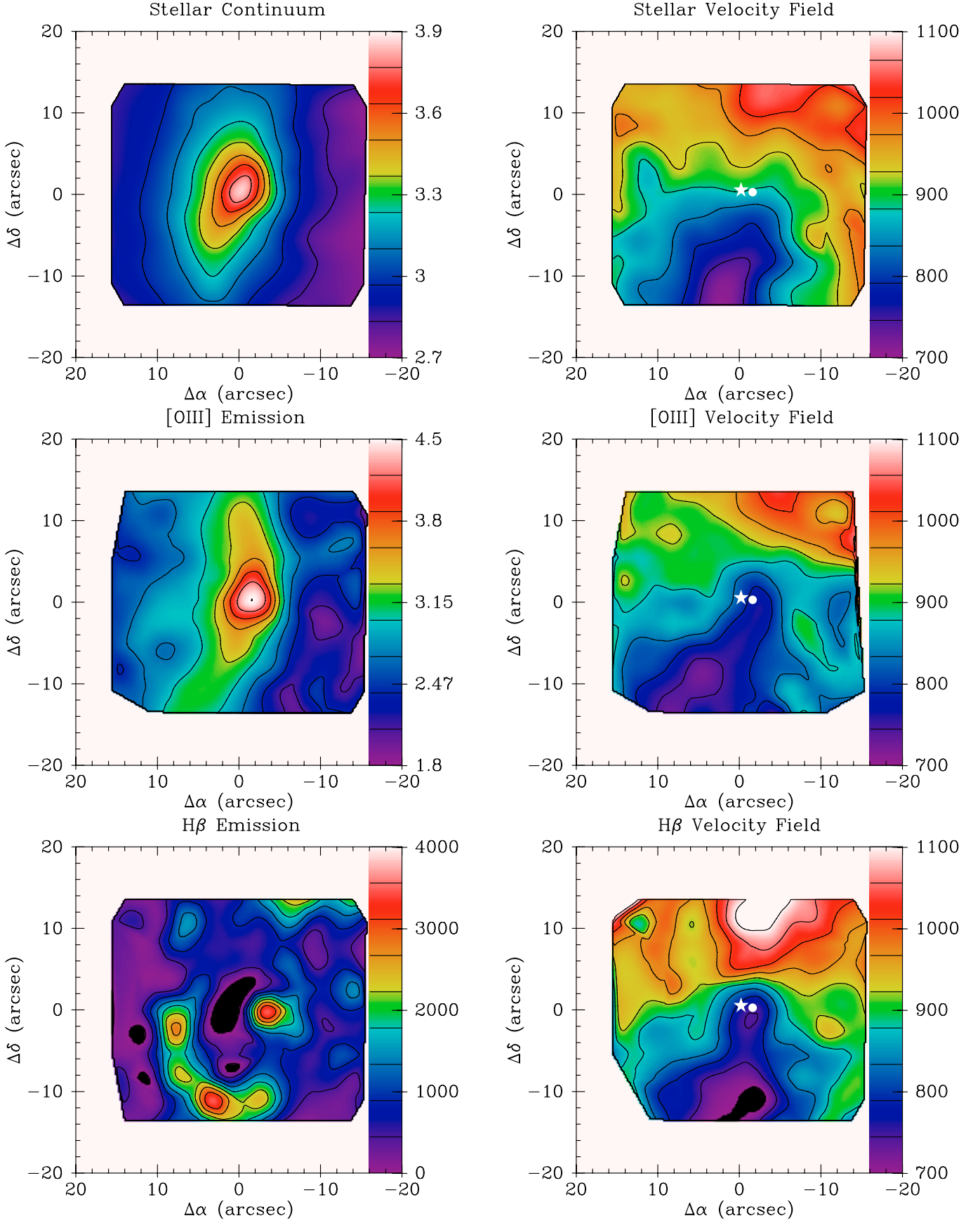
Fig. 1. Intensity (arbitrary units) and velocity (km s ^{-1} ) maps for NGC 5033 (see text). The intensity maps correspond to the stellar continuum (integrated in the \sim 4700 Å–5840 Å wavelength interval), the [OIII] \lambda 5007 and H \beta emission. The star and the circle in the velocity maps represent, respectively, the location of the intensity peak in the stellar continuum and [OIII] intensity maps.
