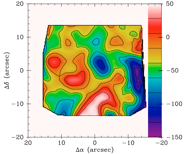
Fig. 8. Residual velocity field obtained subtracting the stellar velocity map from the [OIII] velocity map.
