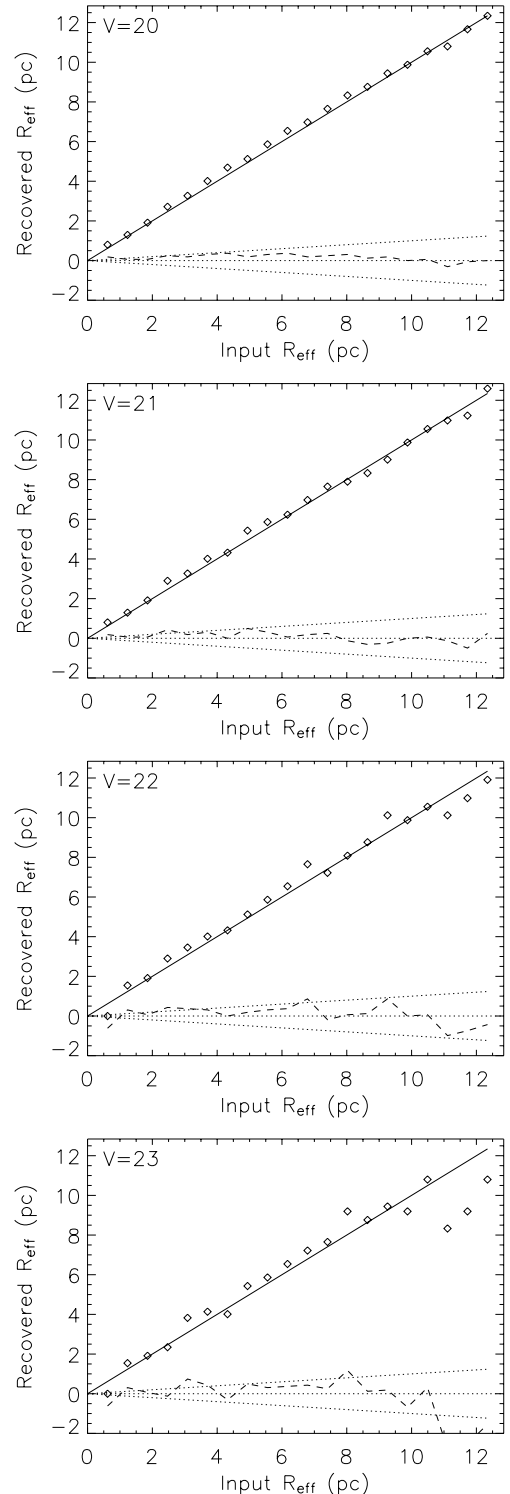
Fig. 15. A test of the accuracy of the measurements of cluster radii. The derived effective radius as a function of both the input effective radius and the magnitude. A one-to-one relation is shown by the solid line. The difference between the recovered and the input radii is shown as the dashed line, while the dotted lines show the value 10% difference between the input and the recovered radii.
