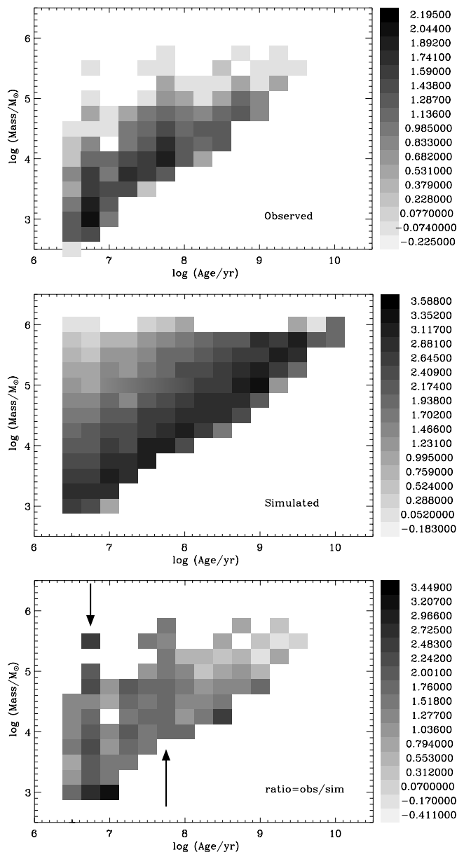
Fig. 11. Top a): The present mass as a function of age for the 1152 clusters that pass our selection criterion. The shading represents the logarithmic number density, with the scale given on the right. Middle b): Same as a) , but for the simulated cluster sample with a constant cluster formation rate (see Sect. 4.3 for details). Bottom c): The ratio between the observed distribution ( top ) and the predicted distribution ( middle ). The arrows indicate two age bins which have an overdensity of clusters relative to the simulated cluster sample.
