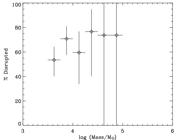
Fig. 14. The fraction of the young (<10 Myr old) clusters per mass bin that are expected to disrupt within the next \sim 10 Myr.
