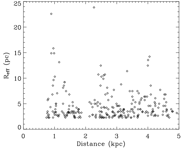
Fig. 20. The effective radii of a clusters versus their distance to the nucleus of M 51. No trend is apparent in the data.
