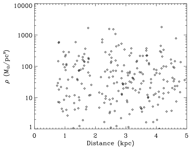
Fig. 21. The density of the clusters versus their distance to the nucleus of M 51. No trend is apparent in the data.
