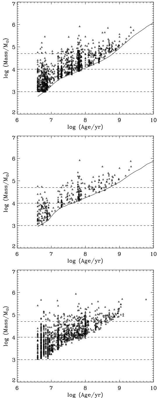
Fig. 10. Top: the present mass as a function of age for the 1078 clusters that pass our \sigma criterion and which have a present mass greater than 1000 M_{\odot} . The solid line is the predicted detection limits using the GALEV models, for m(F439W) = 22.6 mag. The horizontal dashed lines represent constant mass cutoffs used in Fig. 12. Middle: the same as above, but only for those clusters with measured sizes greater than 2 pc. The solid line is the predicted detection limit for m(F555W) = 22.0 mag. Bottom: the present mass as a function of age while leaving metallicity run as a free parameter.
