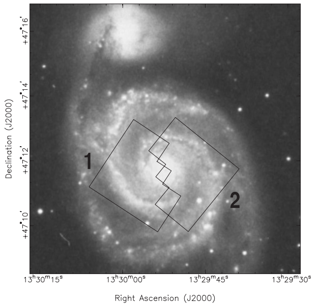
Fig. 1. The orientation of the two HST pointings for the F336W , F439W , F555W , F675W , F814W , and F656N filters overlaid on a Digital Sky Survey image of M 51. North is up, and east is to the left. The left orientation/pointing is referred to as field 1, while the right is referred to as field 2.
