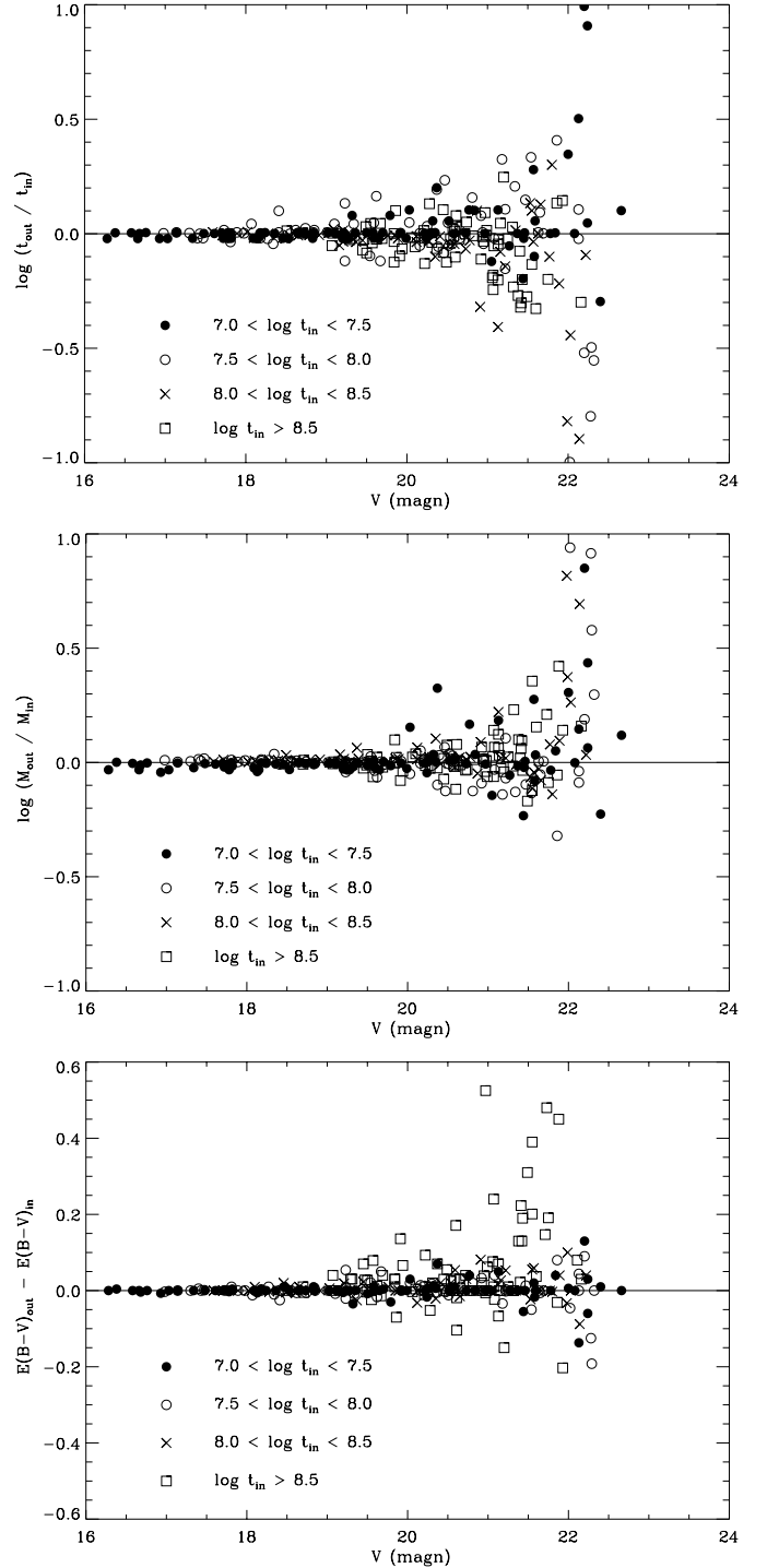
Fig. 5. Comparison between input and output values of the ages ( upper panel, a ), masses ( middle panel, b ) and extinction values ( lower panel, c ) of the synthetic cluster sample. Different symbols indicate different age ranges.
