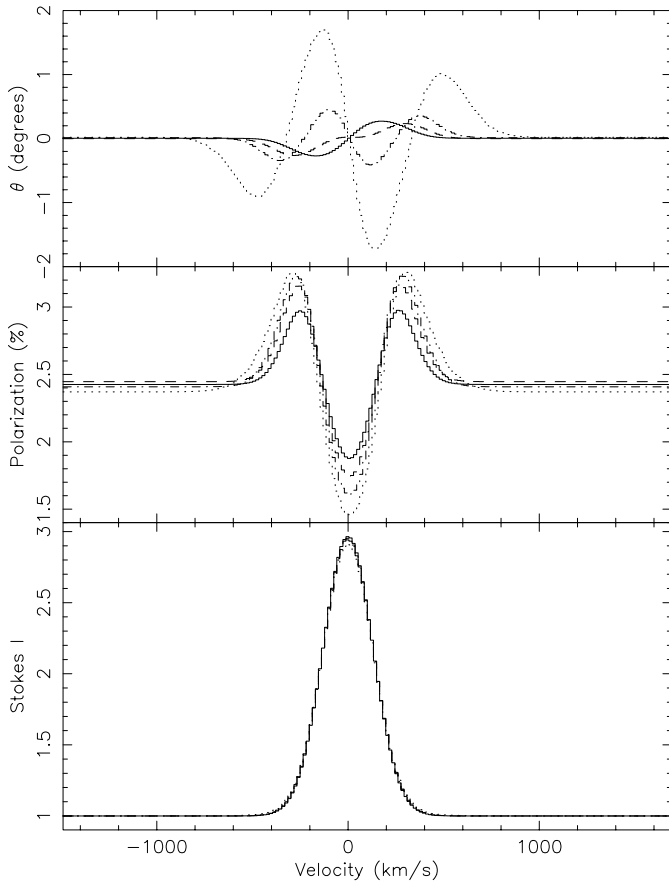
Fig. 4. Varying the size of the disk inner edge: R_{\text{in}} = 1, 2, 3 and 5 R_* for an inclination of 45^\circ . The dotted line is for the model R_{\text{in}} = 1 R_* (the undisrupted disk), which has the largest PA amplitude.
