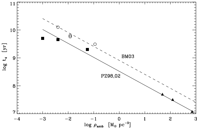
Fig. 2. The predicted dependence of the disruption time, t_4 , of clusters of initial mass of 10^4 M_\odot on the mean ambient density, \rho_{\text{amb}} . The symbols refer to N -body simulations; filled squares are from Portegies Zwart et al. (1998, from left to right models IR16, IC16 and FH16), filled triangles are calculations for star clusters near the Galactic center from Portegies Zwart et al. (2002, from left to right models R150W4, R90W4 and R34W4). The open circles represent models from BM03 (from left to right models V, I, II and IV with 16 384 stars). The dashed line is the relation predicted by BM03, Eq. (8), and the full line is the relation predicted by Portegies Zwart et al.
