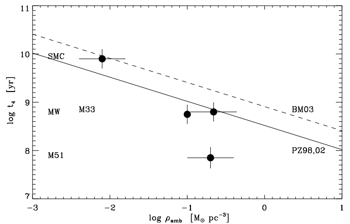
Fig. 4. Comparison between the observed (large dots) and predicted (lines) disruption time t_4 of clusters with an initial mass of 10^4 M_\odot as a function of the mean density \rho_{\text{amb}} in M_\odot \text{pc}^{-3} of the host galaxy. The solid curve present the predictions by Portegies Zwart et al. (1998, 2002) and the dashed line by BM03.
