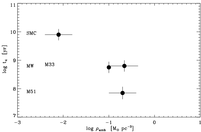
Fig. 3. The relation between the measured values of the disruption time t_4 of clusters with an initial mass of 10^4 M_\odot and the mean ambient density \rho_{\text{amb}} in M_\odot \text{pc}^{-3} , of the galaxies at the galactocentric distances where the studied clusters were located.
