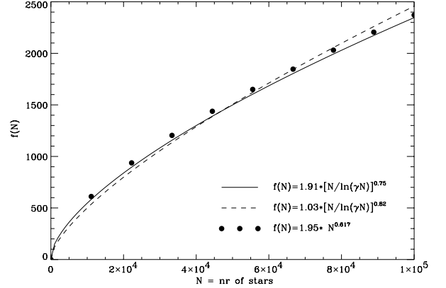
Fig. 1. The function \beta\{N/\ln(0.02N)\}^x of Eq. (6) for the two combinations of \beta and x for clusters with W_0 = 5 (solid line) and 7 (dashed) from BM03 and the power law approximation 1.95 N^{0.617} (dots).
