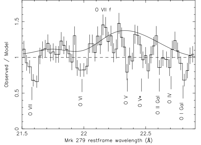
Fig. 7. Chandra LETGS spectrum of Mrk 279 near the oxygen absorption lines. The observed spectrum has been divided by the best fit simple continuum model described in the text (dashed line). The additional broad emission feature is indicated by the curved line. The wavelength scale is for the restframe of Mrk 279 (at z = 0.0306 ). In the line identifications, we have taken into account a small outflow (blueshift) of 300 \text{ km s}^{-1} with respect to this restframe; this outflow has been measured using simultaneous high-resolution UV spectra. A few Galactic absorption lines are labeled with “Gal”.
