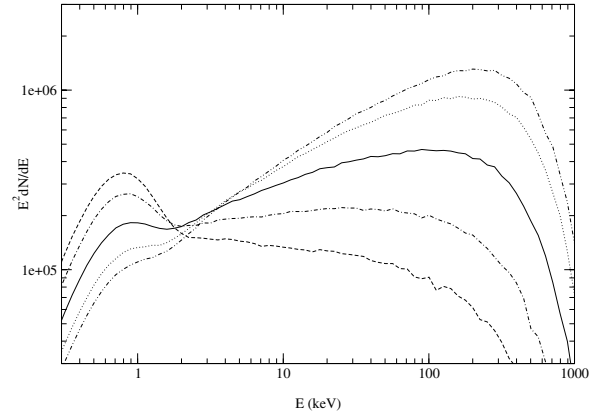
Fig. 3. Emergent photon-number spectra multiplied by E^2 from our jet model for different radii of the base of the jet. Here the dashed, dash-dotted, solid, dotted, and dash-double-dotted curves correspond to R_0/r_g = 30, 50, 100, 200, and 300 respectively. The rest of the parameters are kept at their reference values. The spectra harden as R_0 increases, because the optical depth to electron scattering increases along the direction perpendicular to the axis of the jet. For all the curves, the same number of input photons N = 4 \times 10^6 was used.
