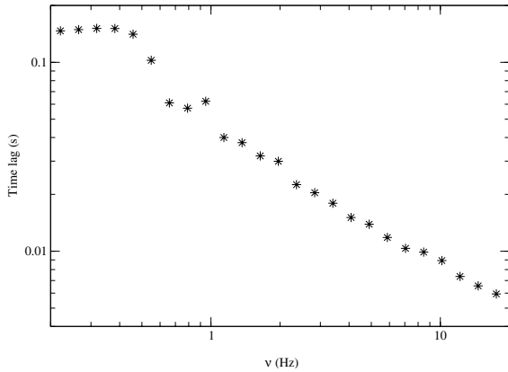
Fig. 4. Computed time lags as a function of Fourier frequency when the reference values of the parameters are used. Positive lags indicate that hard photons lag soft photons. The results are logarithmically rebinned for clarity. The best-fit power law (in the 0.2–20 Hz frequency range) is \nu^{-0.8} .
