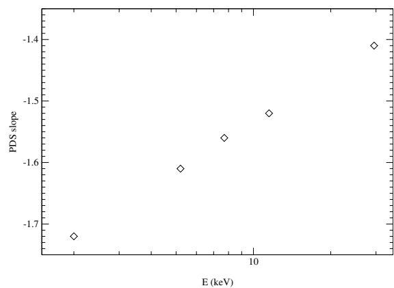
Fig. 8. Power-law slope of the high-frequency power-density spectra (Fig. 7) versus photon energy. The absolute value of the slope for the different energy bands is b_1 : 1.72, b_2 : 1.61, b_3 : 1.56, b_4 : 1.52, b_5 : 1.41.
