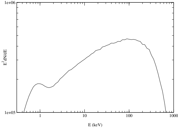
Fig. 1. Emergent photon-number spectrum multiplied by E^2 from our jet model for the reference values of the parameters given in Sect. 3. The soft X-ray excess below 1 keV is essentially the unscattered soft-photon input. When fitted with a power law with an exponential cutoff (see Eq. (6)), we find \Gamma = 1.7 and E_{\text{cut}} = 280 keV.
