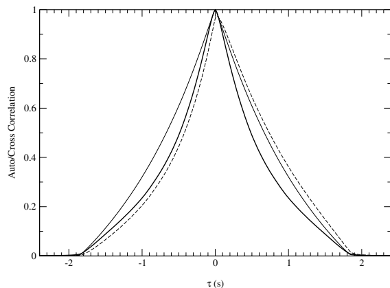
Fig. 6. The autocorrelation functions of the simulated light curves in two energy bands. The thin solid curve corresponds to the soft band (0.2–4 keV), and the thick solid curve to the hard band (14–45 keV). Both curves are normalized to 1 for lag \tau = 0 . Notice that the autocorrelation function becomes narrower in the higher energy band. We also plot (dashed curve) the cross-correlation function of the two light curves.
