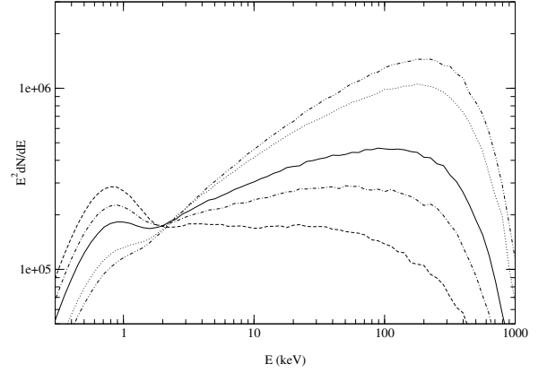
Fig. 2. Emergent photon-number spectra multiplied by E^2 from our jet model for different optical depths \tau_{\parallel} . The dashed, dash-dotted, solid, dotted and dash-double-dotted curves correspond to \tau_{\parallel} = 1.5, 2, 2.5, 3.5, and 4 respectively. The rest of the parameters are kept at their reference values. The power-law slope decreases with increasing optical depth from \Gamma \simeq 2 (for \tau_{\parallel} = 1.5 ) to \Gamma \simeq 1.45 (for \tau_{\parallel} = 4 ). The cutoff energy E_{\text{cut}} varies slowly in the region 260–300 keV. For all the curves, the same number of input photons N = 4 \times 10^6 was used.
