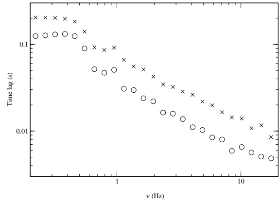
Fig. 5. Computed time lags as a function of Fourier frequency for different dimensions of the jet. The crosses correspond to a large jet with R_0 = 300r_g and z_0 = 20r_g , and the open circles to a smaller jet with R_0 = 50r_g and z_0 = 2r_g . The lags of the bigger jet are a factor of 2 larger than those of the smaller one at the same frequency. In either case, the best-fit power law (in the 0.2–20 Hz frequency range) is \nu^{-0.8} .
