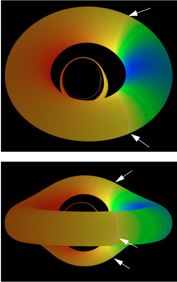
Fig. 5. Images of an accretion torus around a Kerr black hole viewed at inclination angles of 45^\circ (top) and 85^\circ (bottom). The angular momentum of the black hole a = 0.998 . The torus is constructed using the velocity law in Sect. 4.2. The inner and outer radii are determined by the critical surface as described in the same section. High-order images are shown. The energy shift of the emission is represented by a false-colour map laid on the torus surface. Red-shifted emission is coloured yellow/red and blue-shifted emission is coloured blue. The grey lines indicated by the arrows mark the region where the emission has zero energy shift, separating the torus into regions with red and blue shifted emission.
