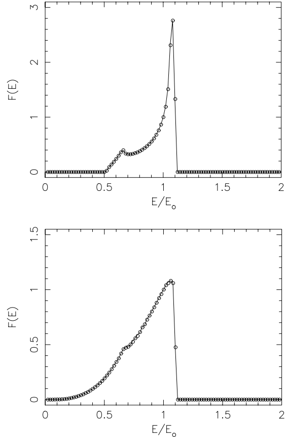
Fig. 3. The profiles of emission lines from thin Keplerian accretion disks around a Schwarzschild black hole ( top ) and a Kerr black hole with a = 0.998 ( bottom ). The line profiles are normalized such that the flux F(E) = 1 at E/E_0 = 1 . The viewing inclination angle is 45^\circ . The inner radius of the accretion disk is at the last stable orbit, and the outer radius is 10R_g . The line emissivity on the disk surface is a power-law which decreases radially outward, and the powerlaw index is -3 . Only emission contributed by the direct disk image is considered; emission from higher-order images is not included. The emission is unabsorbed. In each case, the solid lines correspond to the line profiles obtained by semi-analytic calculations described in Fanton et al. (1997), and the circles represent the line profile obtained by our numerical ray-tracing calculations.
