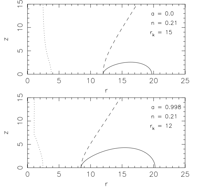
Fig. 1. The critical emitting surface of the torus (solid line), the surface defined by the orbits of marginal stability (dashed line) and the limiting surface where the linear velocity derived from Eq. (54) approaches the speed of light (dotted line) for a Schwarzschild black hole (top panel) and a Kerr black hole with a = 0.998 (bottom panel). In both cases we consider an profile index n = 0.21 (see Eq. (54)), which gives the tori an angular momentum profile similar to those obtained in the accretion disk simulation of Hawley & Balbus (2002). The Kepler radius r_k is 15 for the Schwarzschild black hole and is 12 for the Kerr black hole.
