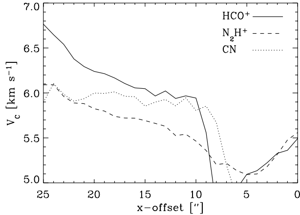
Fig. 14. Velocity field in \text{HCO}^+ , \text{N}_2\text{H}^+ and CN emission: average centroid velocity of the three species in strips perpendicular to the outflow axis across the eastern part of the core.
