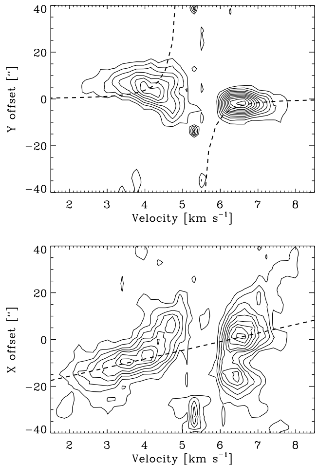
Fig. 9. Position-velocity diagram for the CS emission rotated 12^\circ , so the Y-axis is in the direction of the velocity gradient in the dense material close to the central protostar (see also Fig. 10). The dashed lines indicate Keplerian rotation around a 1.2 M_\odot central object in the upper panel and linear expansion of 0.27 \text{ km s}^{-1} \text{ arcsec}^{-1} in the lower panel.
