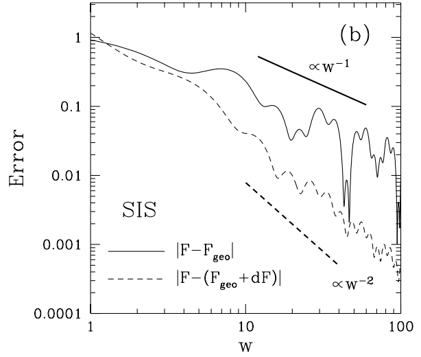
Fig. 2. Same as Fig. 1, but for SIS lens with a source position y = 0.3 .
