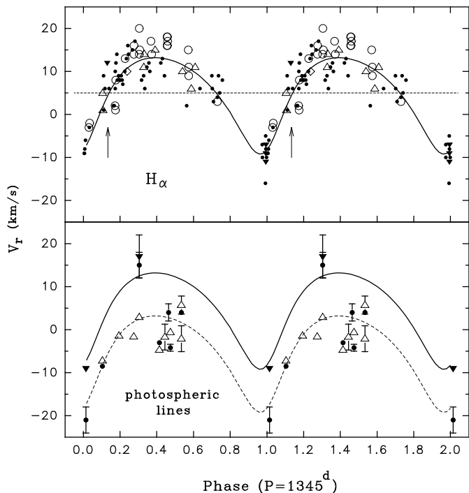
Fig. 5. Top: the bisector velocity V_{\text{bis}} derived at the level 1.5\text{--}2.0 F_c folded with the period P = 1345 days. The least-squares fit to the observations indicated by the solid line illustrates the calculated RV curve. The initial phase corresponds to the epoch of periastron passage. The phase when the observed EW of the H\alpha emission is at maximum is indicated by the arrows. The dashed line corresponds to the \gamma -velocity. Data obtained at different observatories are marked by following symbols: filled circles – Ritter; open circles – CrAO; upward open triangles – OHP; downward filled triangles – SAO; open diamonds – CFHT. Bottom: the RV of the photospheric lines in comparison with the curve calculated for the H\alpha data. The following symbols mark the RV of lines for different elements: filled circles – He I, downward filled triangles – Si II, and upward open triangles – S II. The dashed line indicate the RV curve for the H\alpha data but shifted on -9 \text{ km s}^{-1} .
