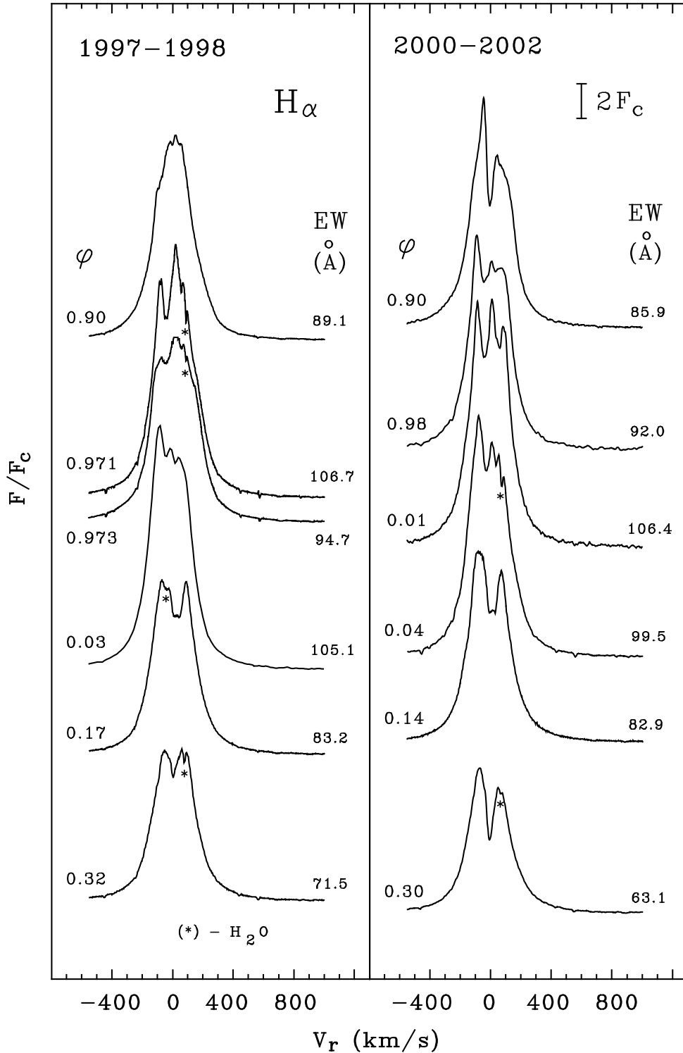
Fig. 1. Typical H\alpha profiles normalized to the continuum ( F_c ) illustrating the evolution of the HD 200775 spectrum in 2000–2002 ( right panel ) in comparison with those observed in 1997–1998 ( left panel ) at similar phases \phi . The water vapor lines near the top of the emission peak are marked by the ( \star ) symbols. The RV scale is given with respect to the star.
