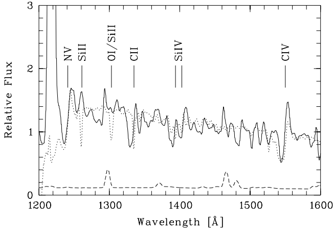
Fig. 4. Low-resolution spectrum of FDF-4691 (solid line) and STARBURST99 spectrum (dotted line). The discrepancy at the interstellar absorption lines (SiII, OI/SiII and CII) is due to the fact that these are not modeled consistently with the extinction by STARBURST99. The dashed line indicates the noise level.
