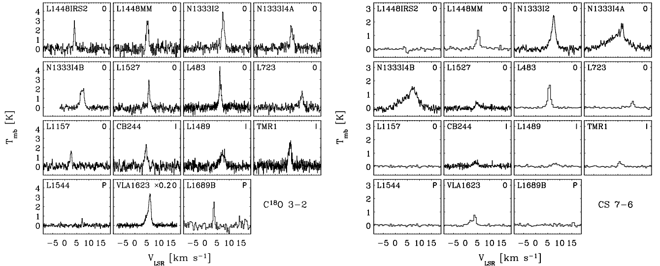
Fig. 1. Spectra of \text{C}^{18}\text{O } J = 3-2 (left) and \text{CS } J = 7-6 (right) from JCMT observations. In this figure, and Figs. 2–4, the classes of the individual objects are indicated in the upper right corner of each plot by “0” for the class 0 objects (envelope mass >0.5 M_{\odot} ), “I” for the class I objects (envelope mass <0.5 M_{\odot} ) and “P” for the pre-stellar cores.
