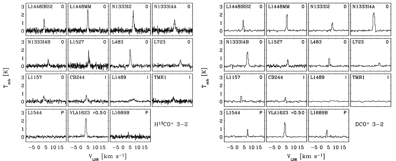
Fig. 2. Spectra of \text{H}^{13}\text{CO}^+ J = 3-2 (left) and \text{DCO}^+ J = 3-2 (right) from JCMT observations.
