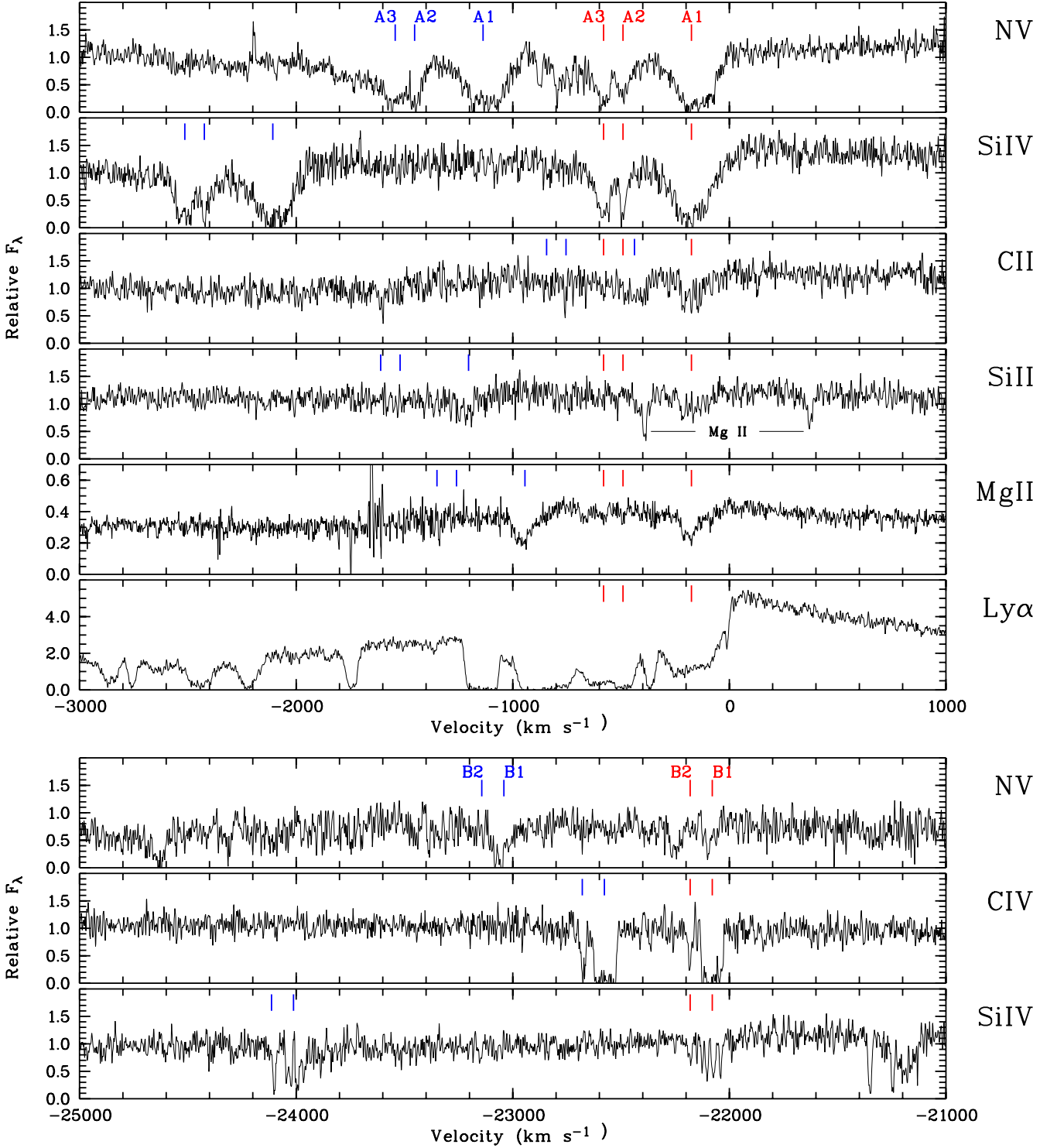
Fig. 2. Portions of the UVES spectrum of SDSS J0011+0055 illustrating the absorption line systems A and B defined in Table 1. System B is best seen in CIV and system A in SiIV (CIV at z \approx 2.29 is outside the observed UVES spectral range). The following transitions are indicated: NV \lambda\lambda 1238.82, 1242.80, CIV \lambda\lambda 1548.20, 1550.78, SiIV \lambda\lambda 1393.75, 1402.77, MgII \lambda\lambda 2796.35, 2803.53, SiII \lambda\lambda 1260.42, 1264.74, 1265.00, CII \lambda\lambda 1334.53, 1335.66, 1335.71, and Ly \alpha \lambda 1215.67. For clarity, the two reddest and very close transitions of SiII and CII are represented by single marks at the mean wavelengths; all four of those transitions are excited-state transitions. Absorption from the high-velocity system B is not detected in SiII or CII, and therefore is not plotted although it lies well within the observed UVES spectral range (SiII \lambda 1260.42 could be present in system B1 but the detection is not convincing). Narrow intervening MgII \lambda\lambda 2796.35, 2803.53 absorption contaminates the SiII absorption of system A2. Narrow intervening CIV \lambda 1548.20 lines are seen slightly longward of the SiIV absorption from system B, along with a broader instrumental artifact. All spectra are plotted on a velocity scale of v/c = (R^2 - 1)/(R^2 + 1) where R = (1 + z_{\text{sys}}) \lambda_0 / \lambda_{\text{obs}} , \lambda_0 the laboratory vacuum rest wavelength of the red transition of the multiplets, and z_{\text{sys}} the systemic redshift of the quasar.
