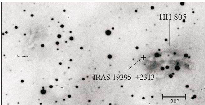
Fig. 9. IRAS 19395+2313 H \alpha : HH 805 and its candidate driving source IRAS 19395+2313.
