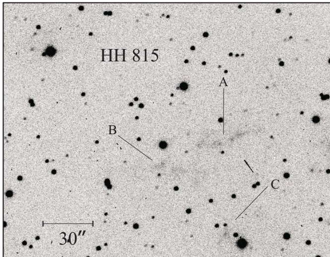
Fig. 15. LkHα 234 [SII] : HH 815, to the northeast of the cluster, is the most distant, known, outlying HH object in this region. Its relative position is seen in Fig. 13.
