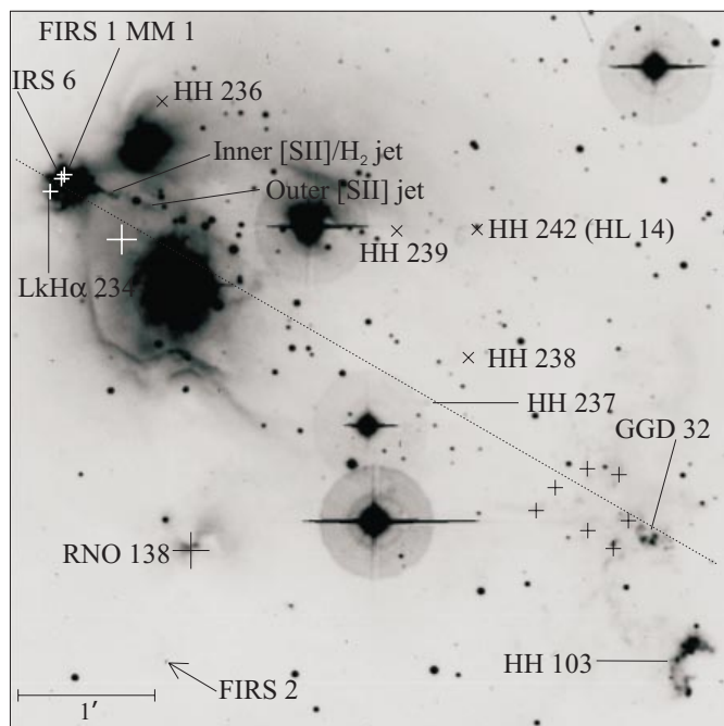
Fig. 14. LkH \alpha 234 [SII]: The cluster region (indicated in Fig. 13) including the “inner” and “outer” optical jets (Ray et al. 1990; Cabrit et al. 1997). The contrast has been changed here with respect to Fig. 13 so that more objects within the cluster core are visible. The white cross to the southwest of LkH \alpha 234 marks the position of IRAS 21814+6552. Black crosses and X’s are used to mark the positions of HH objects found by Eiroa et al. (1992) and Miranda et al. (1993) respectively. The apparent primary outflow axis through the cluster at 60^\circ/240^\circ is marked.
