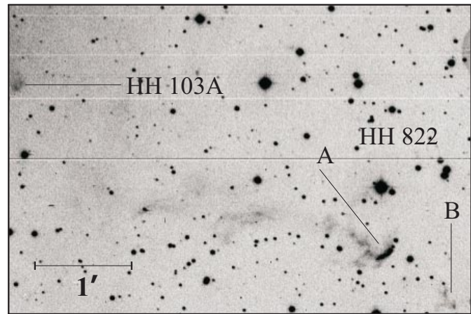
Fig. 17. LkHα 234 [SII] : HH 103 A and HH 822 to the southwest of LkHα 234 .
