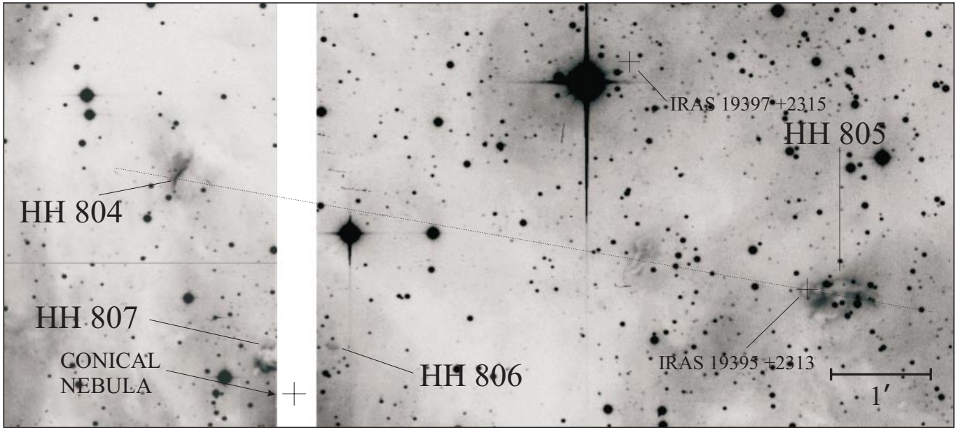
Fig. 8. IRAS 19395+2313 H \alpha : The region around IRAS 19395+2313, including all known additional IRAS sources in its vicinity. Note that IRAS completeness at this distance is \geq 100 L_{\odot} . Four newly discovered HH objects are marked. The position of the conical nebula, visible on the Palomar Sky Survey Red (E) plate and which might be associated with the driving source for HH 806, is indicated. The possible outflow from IRAS 19395+2313 is marked with a dotted line at a PA of 80^{\circ} .
