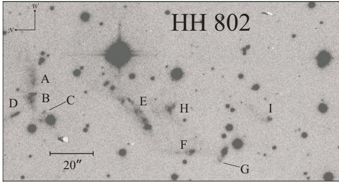
Fig. 3. LkHa 198 [SII] : HH 802, to the southeast of LkHa 198 .
