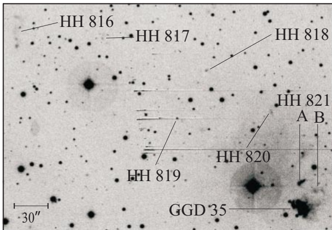
Fig. 16. LkHα 234 [SII] : HH 816–HH 821 (A and B), to the northeast of LkHα 234 .
