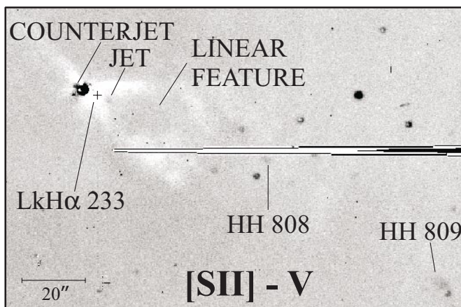
Fig. 12. LkH \alpha 233 [SII] : Continuum subtracted image of the centre of the LkH \alpha 233 nebula. The jet is optically visible here, along with a number of other emission features close to the source including HH 808 and HH 809.
