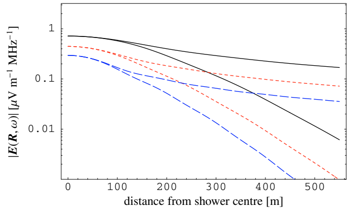
Fig. 14. Radial dependence of |E(\mathbf{R}, 2\pi\nu)| for the maximum of a 10^{17} eV air shower with flaring Agnetta et al. (1997) \Gamma -pdf, R_0 = 4 km and a broken power-law energy distribution from \gamma = 5 –1000. Solid: \nu = 50 MHz, short-dashed: \nu = 75 MHz, long-dashed: \nu = 100 MHz, upper/lower curves for “reduced \theta ” perpendicular/parallel to magnetic field direction.
