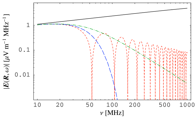
Fig. 6. |E(R, 2\pi\nu)| -spectrum in the centre of the area illuminated by the maximum of a 10^{17} eV air shower with R_0 = 4 km and \gamma \approx 60 . Solid: full coherence, short-dashed: uniform 5.6 m line charge, long-dashed: Gaussian line charge with \sigma = 1.61 m, dash-dotted: asymmetrical \Gamma -distribution with c\sigma_t = 1.61 m.
