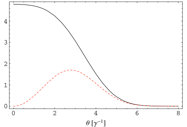
Fig. 3. Comparison of |A_{\parallel}| (solid) and |A_{\perp}| (short-dashed) for \nu = 100 MHz, \gamma = 60 and B = 0.3 G. Absolute scale is arbitrary.
