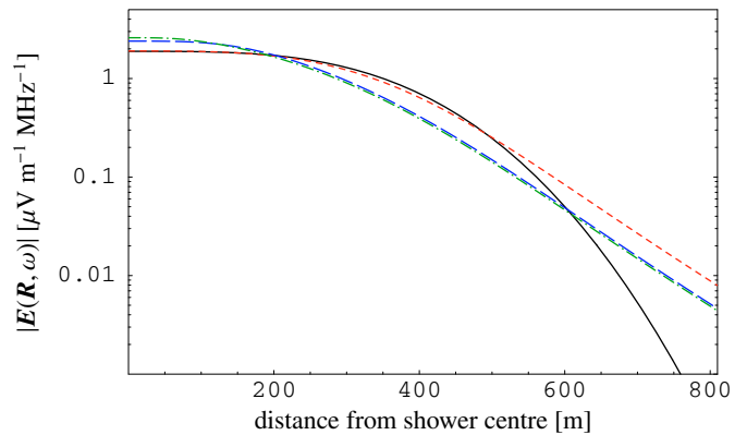
Fig. 7. Radial dependence of |E(R, 2\pi 50 \text{ MHz})| for the maximum of a 10^{17} eV point source shower with R_0 = 4 km for the \gamma \approx 60 case (solid) and for broken power-law distributions from \gamma = 5-120 (short-dashed), \gamma = 5-1000 (long-dashed) and \gamma = 5-10000 (dash-dotted).
