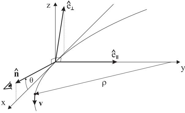
Fig. 1. Geometry of single particle synchrotron radiation for an observer with line-of-sight vector \hat{n} enclosing a minimum angle \theta to the instantaneous particle velocity vector v . The equivalent curvature radius is given by \rho , and the emission can be conveniently divided into the components \hat{e}_\perp and \hat{e}_\parallel . The particle trajectory lies in the x - y plane.
