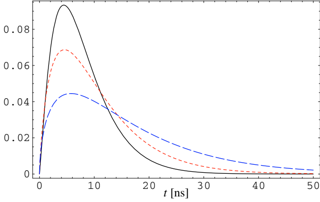
Fig. 4. \Gamma -pdf determining the arrival time distribution of particles as measured by Agnetta et al. (1997). Solid: in the shower centre, short-dashed: 50 m from shower centre, long-dashed: 100 m from shower centre.
