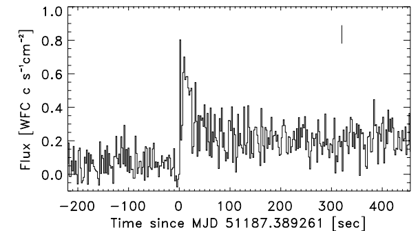
Fig. 3. Light curves obtained with the WFC on January 9–13, 1999 at 300 s resolution ( top panel ) and focused on the burst onset at 2 s resolution ( bottom panel , with vertical line indicating a typical 1\sigma error). The bandpass is 2–28 keV.
