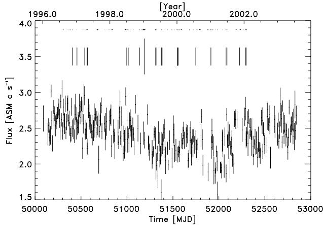
Fig. 1. 2–12 keV RXTE-ASM light curve of 4U 1254-69 at a 1-week time resolution. Data points with errors in excess of 0.2 \text{ c s}^{-1} were excluded from this plot. The horizontal lines in the top indicate the WFC coverage of the source and the vertical lines the bursts detected with the WFC. The long vertical line indicates the time of the superburst.
