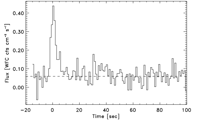
Fig. 2. The average 2–28 keV profile over all normal bursts observed from 4U 1254-69, except the one related to the superburst. The dashed line refers to the persistent flux level.
