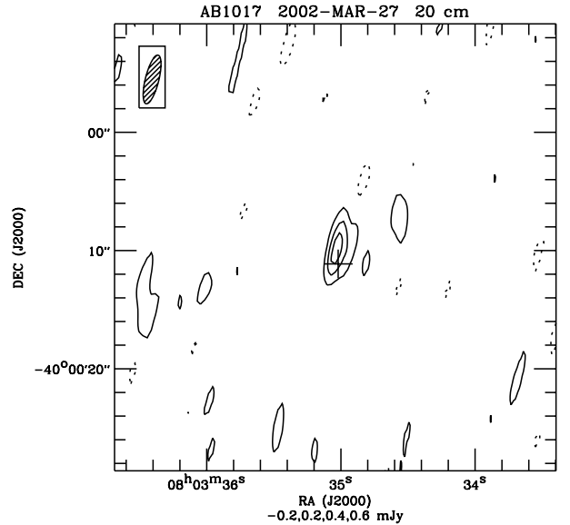
Fig. 4. VLA observation at 20 cm. The contour levels follow a linear scale and the values are listed at the bottom of the figure. The negative contour is given by the dashed line. The first positive contour is at about twice the rms noise in the map. The beam is shown in the upper left corner. The cross indicates the optical ICRS 2000.0 position (from SIMBAD), corrected for proper motion. The \sim 1.4'' offset with the radio position is most probably due to ionospheric refraction, which is more important at longer wavelengths and at the low elevation at which \zeta Pup was observed.
