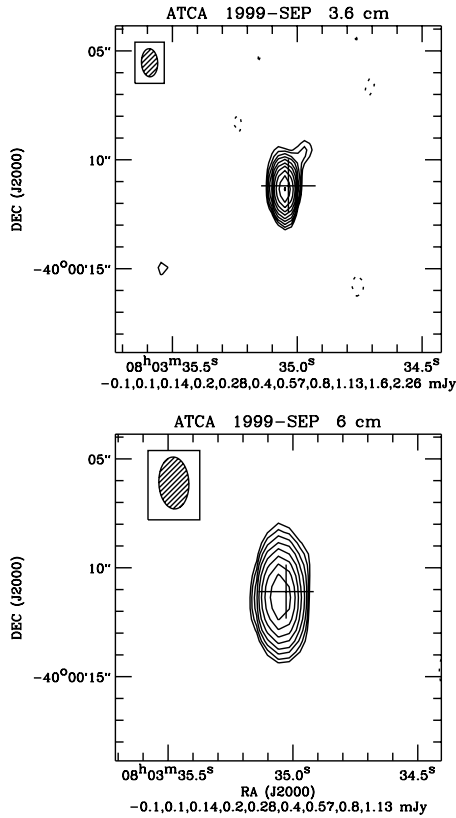
Fig. 3. ATCA observation (all data combined) of \zeta Pup at 3.6 and 6 cm. The cross indicates the optical ICRS 2000.0 position (from SIMBAD), corrected for proper motion (see Table 2). The contour levels follow a logarithmic scale: their values are listed at the bottom of each figure. The negative contour is given by the dashed line. The first positive contour is at about three times the rms noise in the map. The beam is shown in the upper left corner.
