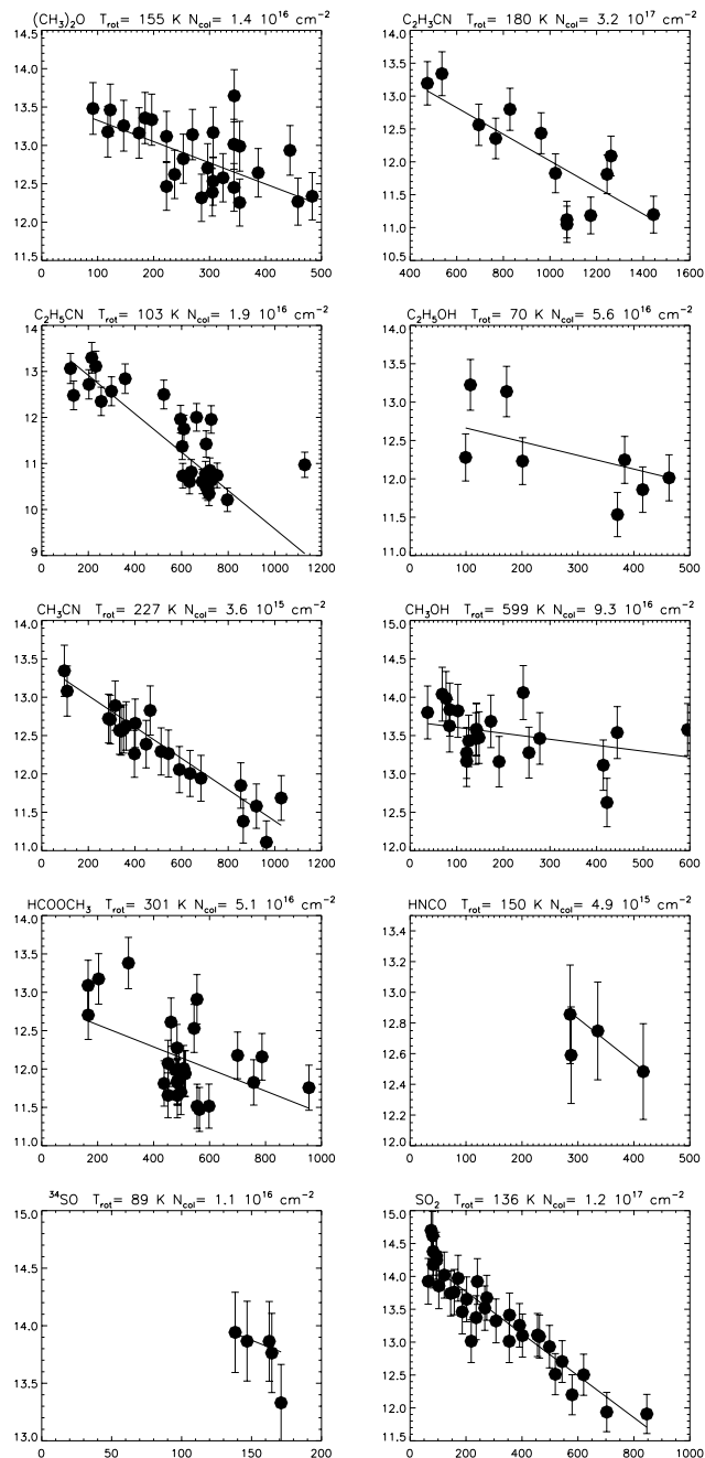
Fig. 7. Rotational temperature diagrams. The fitted lines were derived from a noise-weighted least squares fitting procedure.
