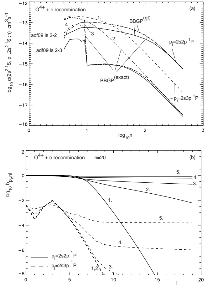
Fig. 2. O^{4+} recombination. a) Partial n -shell recombination coefficients: initial recombining metastable 2s^2 1S , intermediate excited parent p_i , final states (2s^2 1S)n with p_i = 2s2p^1 P and 2s3p^1 P . T_e = 1.6 \times 10^6 K, N_e = N_p = 0 . BBGP (gf) indicates use of standard cor_l matching the GF, BBGP (exact) indicates use of specific cor_l . For the \Delta n = 0 case, BBGP (gf) and BBGP (exact) are superposed. \Delta n = 1 cases: 1. no alternative Auger channels, GF cor_l ; 2. no alternative Auger channels, specific cor_l ; 3. 2s3p^1 P - 2s3s^1 S alternative Auger channel, specific cor_l ; 4. as before and 2s3p^1 P - 2s2p^1 P alternative Auger channel, specific cor_l . b) b_{p_i, nl} factors for doubly-excited states of O^{3+} relative to O^{4+} 2s^2 1S for p_i = 2s2p^1 P and 2s3p^1 P , n = 20 , T_e = 10^6 K, N_e = N_p , plasma Z_{\text{eff}} = 1 . Cases: 1. N_e = 10^{10} cm -3 ; 2. N_e = 10^{12} cm -3 ; 3. N_e = 10^{13} cm -3 ; 4. N_e = 10^{14} cm -3 ; 5. N_e = 10^{15} cm -3 . Note the alternative Auger channel reduction for the p_i = 2s3p^1 P graphs.
