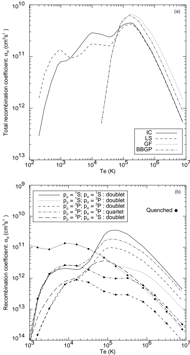
Fig. 1. The graphs contrast \alpha_d^{(\text{tot})}(p_p \rightarrow p_i \rightarrow p_\sigma) vs. T_e for the dielectronic recombination of O^{4+} ions in various approximations at zero density. a) p_p = O^{4+}(2s^2 1S) , p_\sigma = O^{3+}(2s^2 2p^2 P) : \Delta n = 0 and \Delta n = 1 intermediate parents included. The Burgess GF includes only the dipole 2s^2 1S - 2s2p^1 P and 2s^2 1S - 2s3p^1 P transitions. BBGP incorporates specific cor_l correction factors, energies which differ from those implicit in the GF, and the 3p - 3s alternative Auger channel. The level 1 and level 2 results include all allowed and non-allowed parent transitions within the n = 2 and n = 3 complexes. Note the low temperature extension which cannot be modelled with the GF and BBGP. The correct distinction and positioning of the key lowest resonances are possible only at level 2 . b) p_p = O^{4+}(2s^2 1S) and O^{4+}(2s2p^3 P) , p_\sigma = O^{3+}(2s^2 2p^2 P) and O^{3+}(2s2p^2 4P) : level 1 results separated by spin-system and final parent. Recombination from-and-to metastables cannot be handled by the GF. Excited-states built on the 2s2p^3 P parent have a spin-change autoionization pathway. The level 1 metastable-resolved totals do not include this loss. Within an LS-coupled GCR picture using level 1 data, spin-breakdown Auger data is included explicitly in the GCR calculations for the correct linking of systems built on the 2s^2 1S and 2s2p^3 P parents. The relevant final-parent-changing Auger data is included in the adf09 data file specification. For comparison with simpler treatments, totals including quenching of n -shells > 4 built on the 2s2p^3 P parent are also shown.
