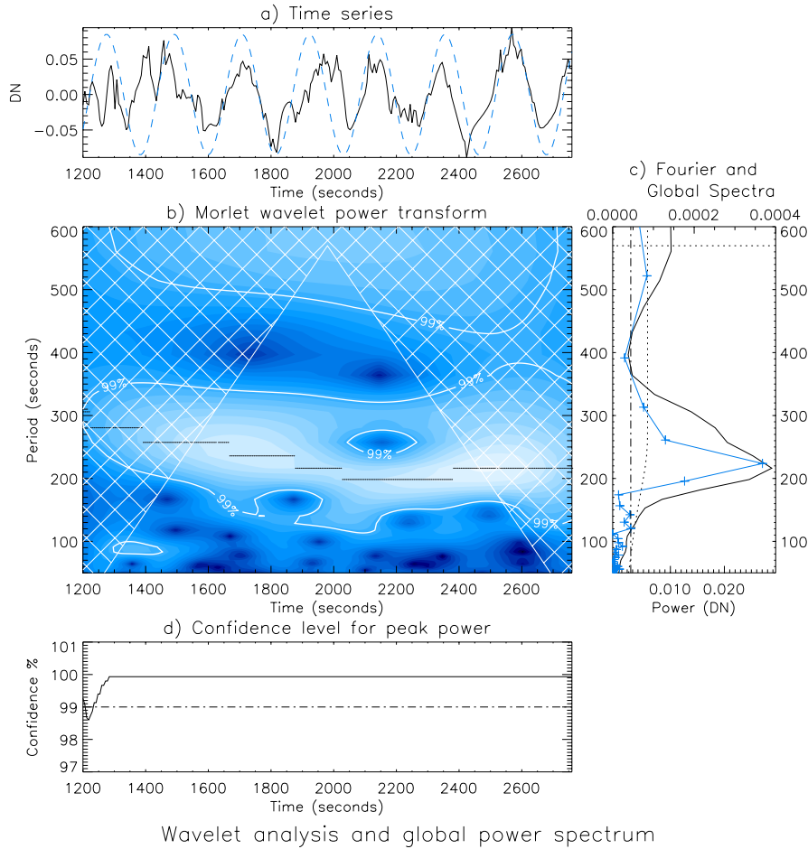
Fig. 2. a) The filtered timeseries used for our analysis b) The Morlet wavelet power transform of the post-impulsive phase part of the August 1989 II Peg flare. Period is plotted as a function of time from the beginning of the entire time series. Contours are computed by defining the power, at each period, at which detections are 99% confident using a \chi^2 distribution with two degrees of freedom. c) Summation of the wavelet power transform over time (full line) and the Fast Fourier power spectrum (crosses) over time, plotted as a function of period. Both methods have detected a well pronounced 220 s oscillation. The global Wavelet (dotted line) and Fourier (dashed dotted line) 99% significance levels are also plotted. Periods above the horizontal line (dotted) fall within the COI. d) The confidence levels for the frequency that contains the greatest power, dark lines in b) , are plotted as a function of time (full line).
