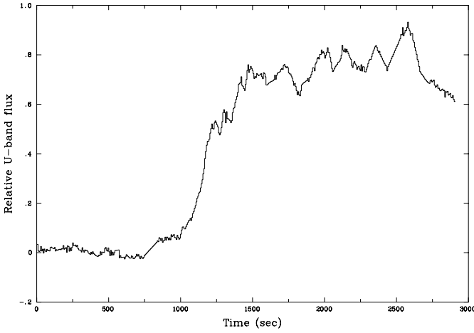
Fig. 1. U -band lightcurve of the II Peg flare. Time is given in seconds since 01:30 UT of 17 August 1989.
