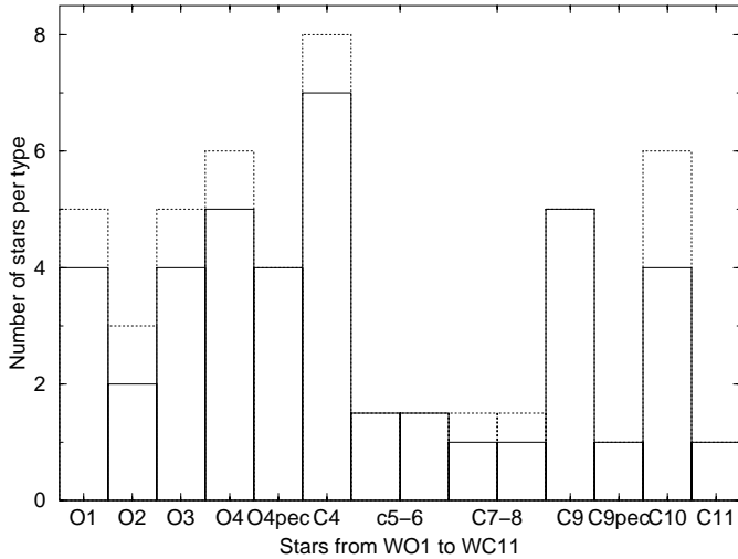
Fig. 11. Histogram of the distribution of our sample (42 stars, solid line), similar to the distribution of the whole well-classified sample (50 stars, dotted line).
