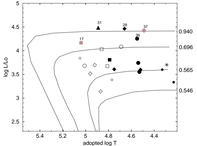
Fig. 10. Positions of the stars on the HR diagram, using symbol legend from Fig. 8. Four evolutionary tracks from Blöcker (1995), for the masses 0.546, 0.565, 0.696 and 0.940 M_\odot , are shown in solid lines.
