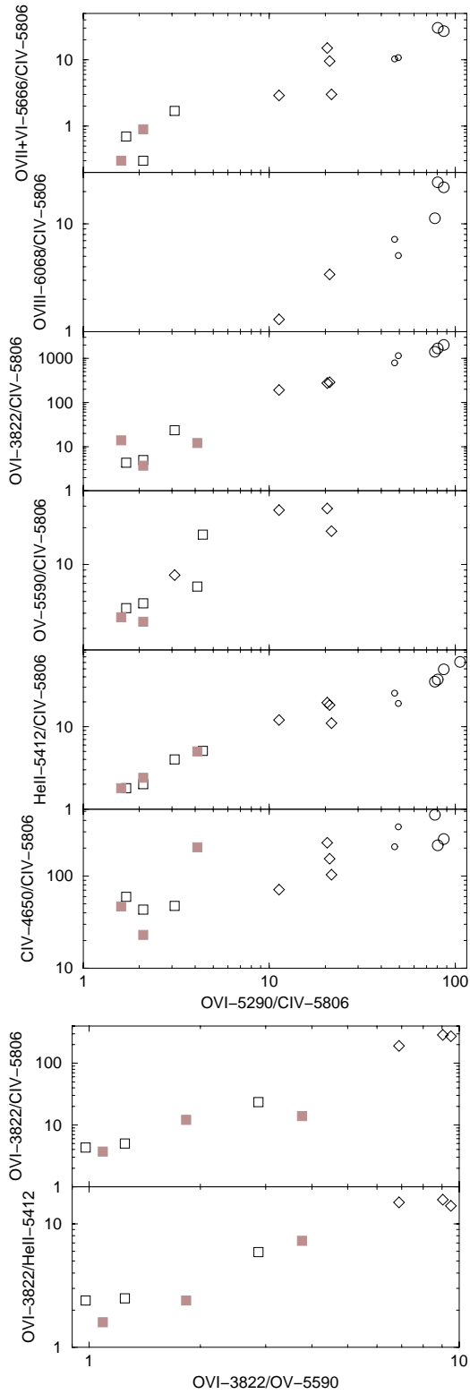
Fig. 5. For hot [WO] stars, top panels: relative variation versus OVI -5290 of the O VII+VI-5666, O VIII-6068, O VI-3822, O V-5590, He II-5412 and C IV-4650 dereddened line intensities. Bottom panels: relative variation versus O VI-3822/O V-5590 of the O VI-3822/C IV-5806 and O VI-3822/He II-5412 dereddened line intensities. All line intensities are relative to C IV-5806 = 100. See symbol legend in Fig. 3.
