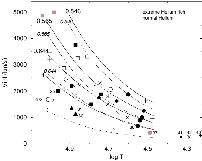
Fig. 9. 42 CSPNe plotted on the tracks from Pauldrach et al. (1988). See the symbol legend in Fig. 8. The data points from Pauldrach et al. (1988) are also shown with the symbols “+” and “x”.
