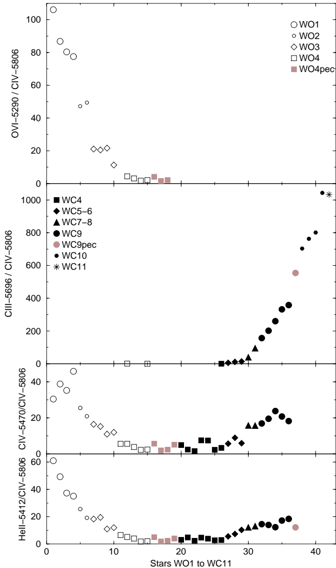
Fig. 3. Upper panels: variation along the [WO] and [WC] types of the O VI-5290/C IV-5806 (early-types) and C III-5696/C IV-5806 (late-types) dereddened line ratios. Lower panels: variation of the CIV-5470/C IV-5806 and He II(C II ? )-5412/C IV-5806 dereddened line ratios. The numbers 1 to 42 on the abscissa correspond to the observed stars (see Table 3). All line intensities are relative to C IV-5806 = 100.
