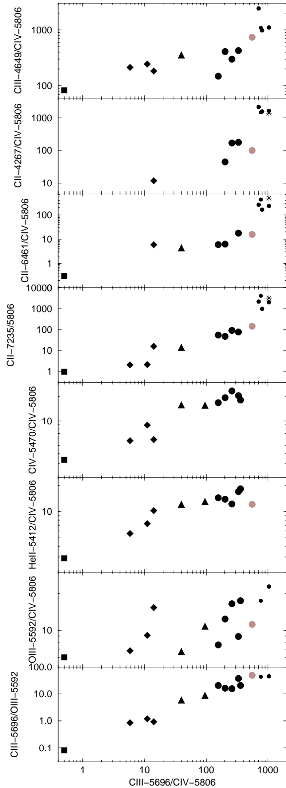
Fig. 6. For [WC] stars, relative variation versus C III-5696 of the C III-4649, C II-4267, -6461, -7235, C IV(C II?) -5470, He II(C II?) -5412 and O III-5592 dereddened line intensities, and of the C III-5696/O III-5592 ratio. All line intensities are relative to C IV-5806 = 100. See symbol legend in Fig. 3.
