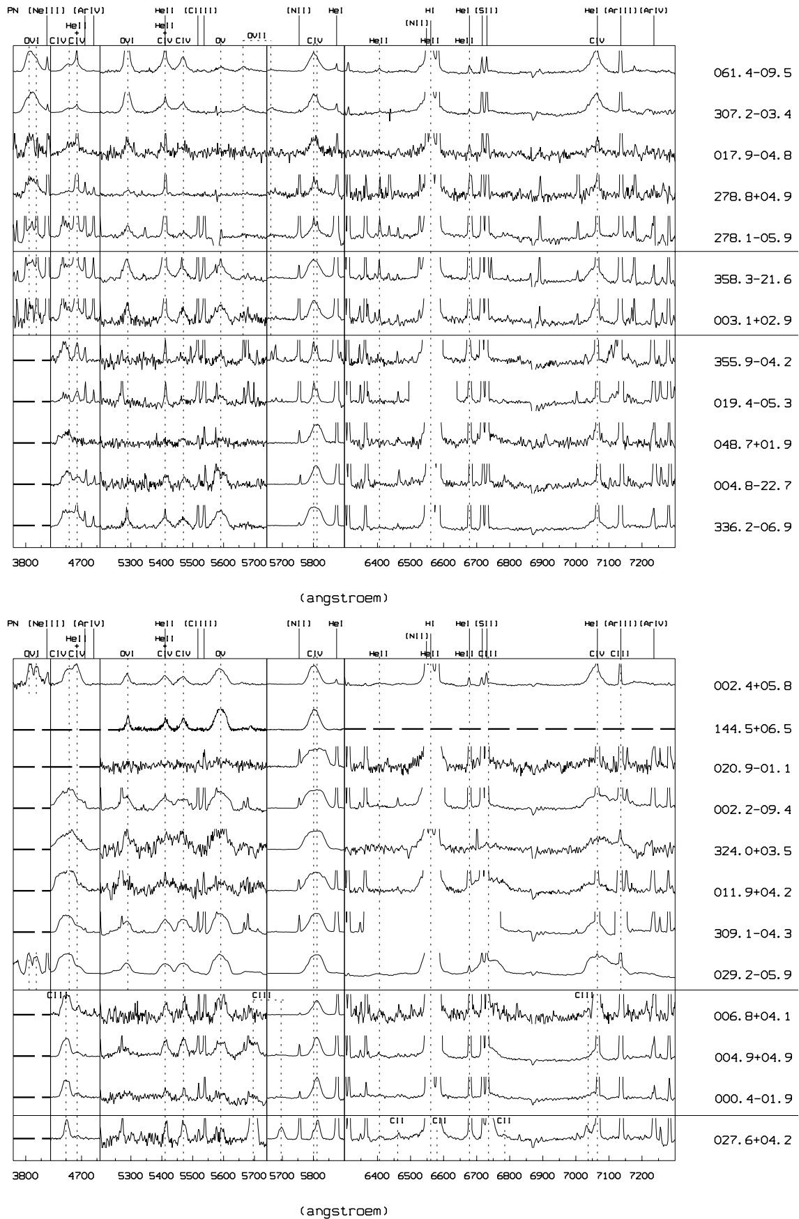
Fig. 1. Spectra of 36 WR CSPNe stars (see Tables 1a and 3) ordered according to the evolutive sequence. The 5200–5670 Å range has been zoomed, in order to better distinguish the different emission lines. Nebular lines are shown at the top of the figures.
