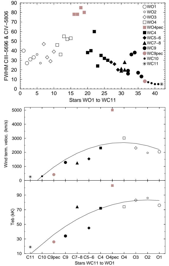
Fig. 8. Upper panel: variation of the FWHM of C IV-5806 and C III-5696 along the spectral sequence, averaged from Table 1a. Middle and lower panels: variation of the mean terminal wind velocity and the stellar temperature ( T_{\text{eb}} ), respectively, through the spectral sequence from the [WO1-4] to [WC4-11] subtypes. The fits (solid line) include the [WO4]pec point.
