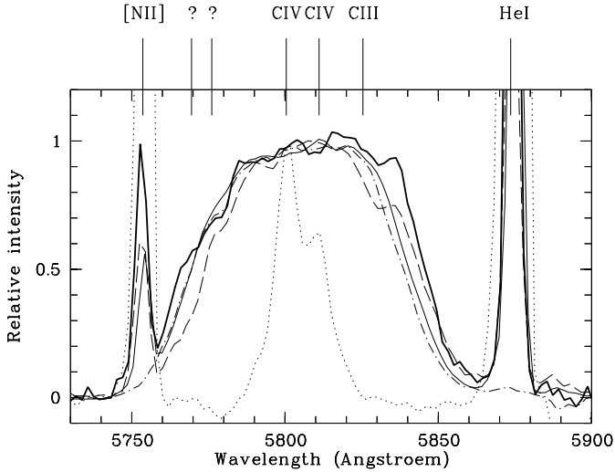
Fig. 7. C IV-5801/12 superimposed line profiles of the four [WO4]pec stars. The thick profile corresponds to M 1-51 (20.9-1.1), and the thin solid line to Cn 1-5 (2.2-9.4). M 1-32 (11.9+4.2) and PM 1-89 (324.0+3.5) are represented with a dashed and dashed-dotted line respectively. For comparison, the C IV line profile of the wels star M 1-61 (19.4-5.3) has been added (dotted line).
