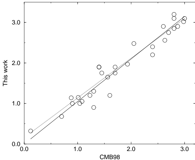
Fig. 2. Comparison of the dereddened line strengths relative to C IV-5806 = 100 given in this work and in CMB98. The resulting correlation seems to be linear: this work = 1.05 \times \text{CMB98} with R^2 = 0.91 (solid line). An alternative fit gives: this work = 0.98 \times \text{CMB98} + 0.16 (dotted line).
