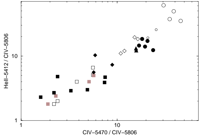
Fig. 4. Correlation between the CIV-5470/C IV-5806 and He II-5412/C IV-5806 dereddened line ratios. All line intensities are relative to C IV-5806 = 100. See symbol legend in Fig. 3.
