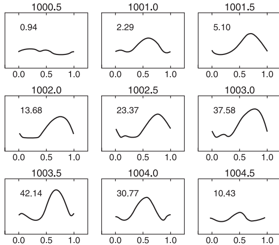
Fig. 2. Estimated orbital light curves from superhump dissipation pattern projected for an observer at high inclination for 9 different superhump phases from Murray’s (1999) simulation. Horizontal axis: orbital phase; vertical axis: intensity in arbitrary units; number on top: time elapsed in simulation in units of orbital period /2\pi ; number inside frame: strength of dissipation (arbitrary unit).
