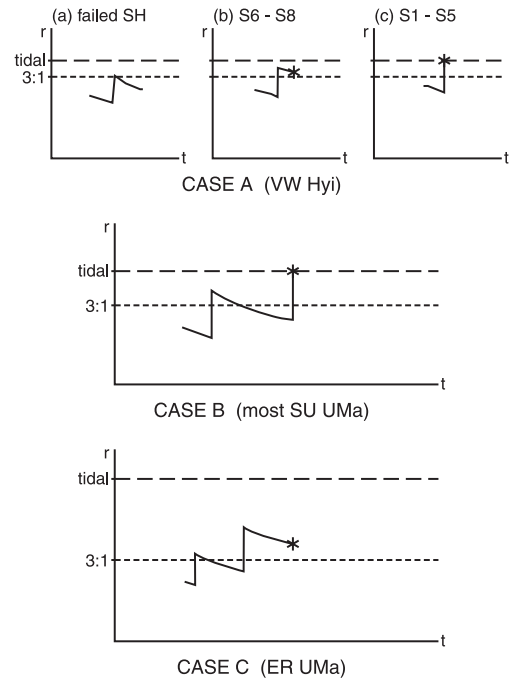
Fig. 4. Various ways in which superoutbursts are triggered (see text for details). Horizontal axis: time, vertical axis: radius. Short dashed line: 3:1 resonance radius, long-dashed line: tidal truncation radius, solid line: outer disk radius, asterisk: ignition of superoutburst. In order of decreasing mass ratio (increasing separation of tidal and 3:1 resonance radii, increasingly longer growth time of superhumps): case A: relatively large mass ratio around 0.2 (a), (b), and (c): ordinary outbursts occurring in various stage of readiness for a superoutburst in one and the same system. Case B: smaller mass ratio. Case C: extremely small mass ratio.
