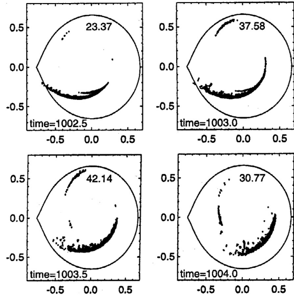
Fig. 1. Superhump dissipation pattern (black dots) in hydrodynamic simulations for four different superhump phases around superhump maximum. Axes: Cartesian coordinates in orbital plane in units of binary separation. Contour line: primary Roche lobe; time: time elapsed in simulation in units of orbital period /2\pi ; number within Roche contour: strength of dissipation (arbitrary unit). After Murray (1999).
