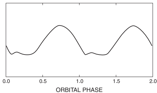
Fig. 3. Superposition of the nine light curves of Fig. 2 weighted by their relative dissipation strength. Horizontal axis: orbital phase; vertical axis: intensity (arbitrary unit). This corresponds to a synchronous summation at the orbital period of observed superhump light curves.
