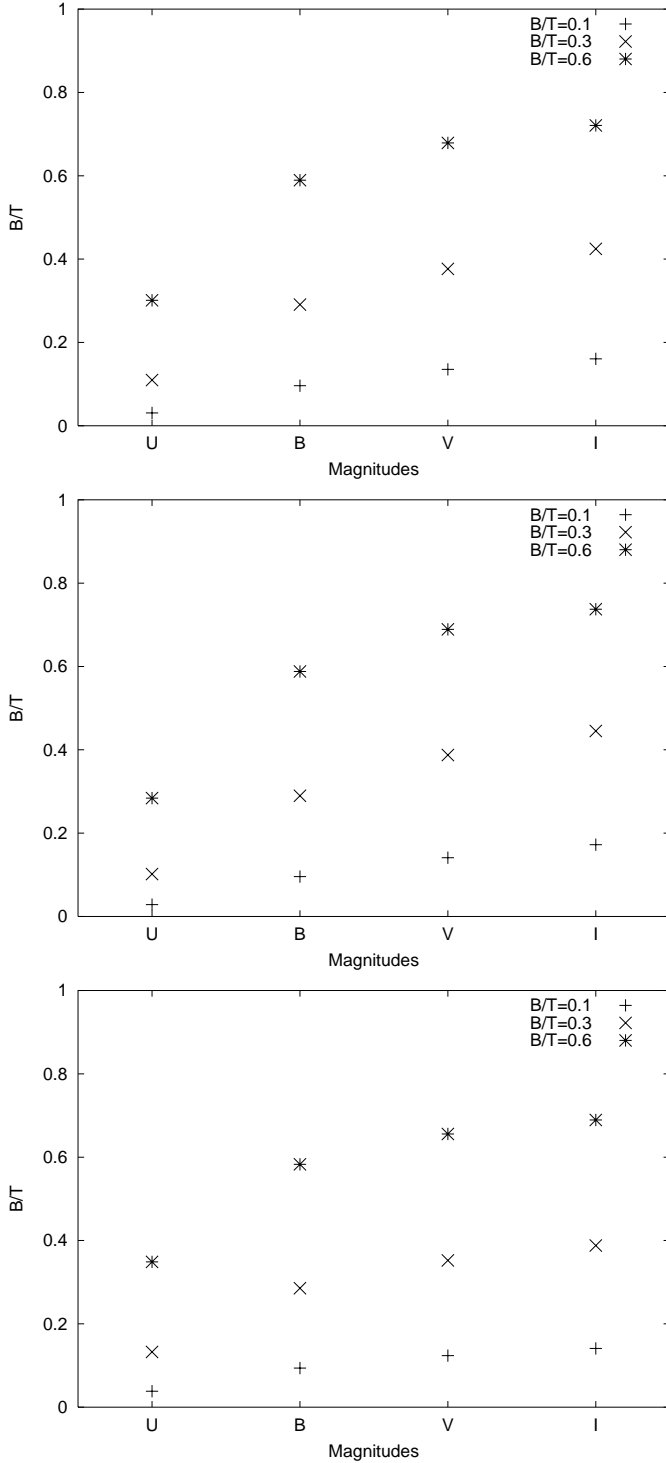
Fig. 3. Present-day B/T -ratios in different filters for model galaxies with (B/T)|_B = 0.1, 0.3, and 0.6 , respectively. Top panel: equal age components, middle panel: old bulge and younger disk, bottom panel: old disk and younger bulge.
