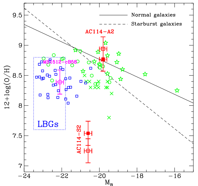
Fig. 6. Oxygen abundance ( 12 + \log(O/H) ) as a function of B -band absolute magnitude. The metallicity–luminosity relations for nearby “normal” (solid line; Kobulnicky & Zaritsky 1999) and starburst (dashed line; Mouhcine & Contini 2002; Melbourne & Salzer 2002) galaxies are shown. The location of the two z \sim 1.9 galaxies S2 and A2 in the lensing cluster AC 114 is shown without extinction correction (empty squares) and assuming a reddening E(B-V) = 0.3 and 0.4 for S2 and A2 respectively (filled squares). We show for comparison samples of intermediate-redshift galaxies: UV-selected galaxies at z \sim 0.1-0.4 (circles; Contini et al. 2002), emission-line galaxies at z \sim 0.1-0.5 (stars; Kobulnicky & Zaritsky 1999), and at z \sim 0.5-0.7 (crosses; Hammer et al. 2001). The location of high-redshift ( z \sim 3 ) Lyman break galaxies (LBGs) is shown as a blue box encompassing the range of O/H and M_B derived for these objects (Pettini et al. 2001). High-redshift ( 1.4 < z < 3.4 ) galaxies with oxygen abundances and B -band magnitudes derived from rest-frame UV spectra (Mehlert et al. 2002) are shown as blue squares.
