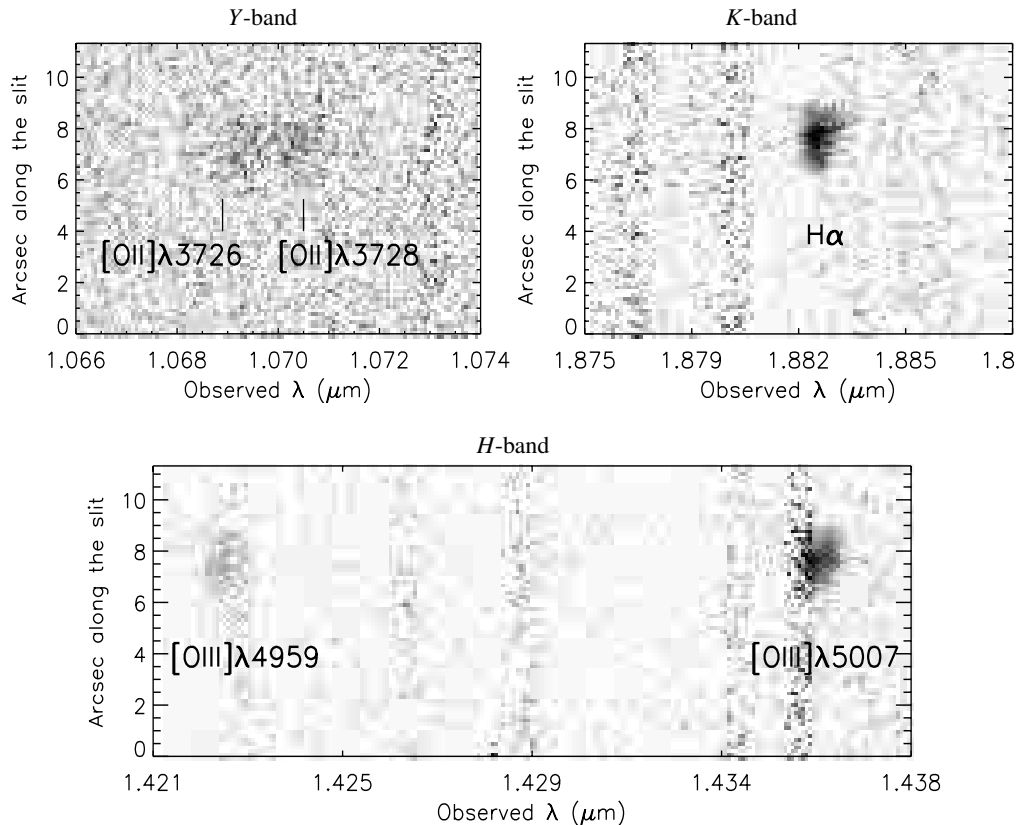
Fig. 2. Two-dimensional images of the ISAAC spectra of AC114-S2 in the Y (1.0 to 1.1 \mu\text{m} ), H , and K bandpasses. Positions of the nebular emission lines are labeled.
