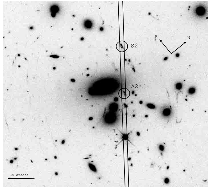
Fig. 1. HST/WFPC2 image ( R -band/ F702W ) of the core of AC114. The position of the ISAAC slit used in our observations is displayed. Circles mark the position of the high redshift galaxies AC114-S2 and AC114-A2.
