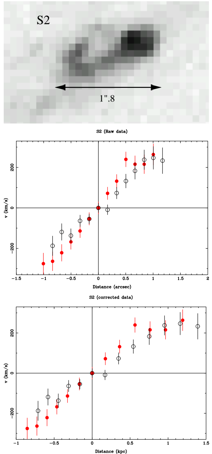
Fig. 5. Spatially resolved emission lines in AC114-S2. Top panel: HST/WFPC2 ( R -band/ F702W ) close image of the lensed galaxy AC114-S2. Mid panel: Raw velocity profiles (in \text{km s}^{-1} ) versus angular distance (in arcsec), as measured on the 2D spectra from the central velocities of H \alpha (open dots) and [O III] \lambda 5007 (full dots) emission lines. Bottom panel: lens corrected velocity profiles.
