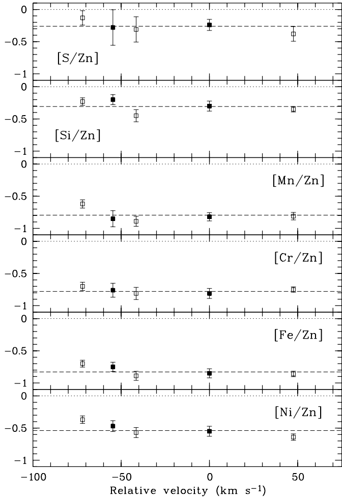
Fig. 7. Depletion of heavy elements relative to Zn in the velocity sub-systems where C I is detected. The metal components at z_{\text{abs}} = 1.96203 , 1.96212 and 1.96225 (see Table 3) are considered as a single sub-system at z_{\text{abs}} = 1.96221 ( V = 0 km s -1 ). The horizontal dashed lines show the column density weighted-mean values of the ratios. Although the depletion pattern is similar in every sub-systems, only two of them (shown as filled squares) have detectable H 2 lines: this demonstrates that the presence of H 2 is not only related to the dust-to-metal ratio.
