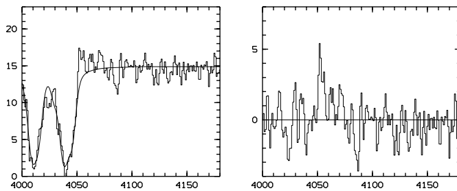
Fig. 3. Left: section of the spectrum with Ly \alpha absorption lines. Note the poor fit to the extreme right wing of the second line. Right: residual after subtraction of the fit shown to the left. A narrow Ly \alpha emission line is now clearly visible. The vertical scale in both plots is in units of 10^{-17} erg s ^{-1} cm ^{-2} Å ^{-1} .
