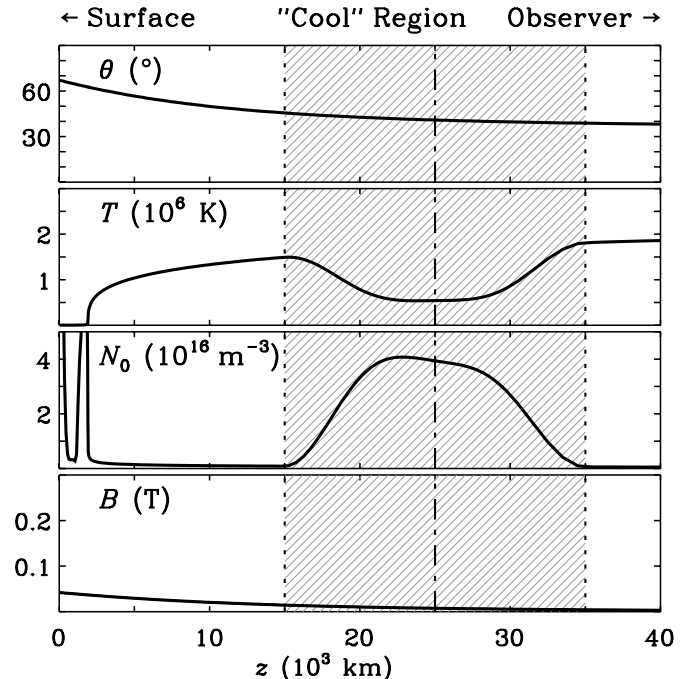
Fig. 6. Same as Fig. 5, but for the extended thermal source (EXTS) with (evaporated) cooler and more dense plasma inside the hatched region with thickness L = 20000 km centered at z = 25000 km.
