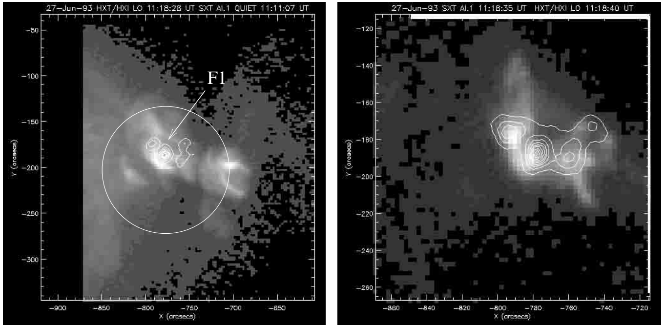
Fig. 4. Left: Yohkoh HXT 14–23 keV hard X-ray sources at 11:18:28 UT (contours) over the Yohkoh SXT soft X-ray image at 11:11:07 UT. “F1” points to the location where the soft X-ray flare started and most of the hard X-ray emission was coming from before Yohkoh night time set in. The white circle represents the Metsähovi 2.4 arcmin radio beam, pointed to the active region and recording the total flux density from that area. Right: Yohkoh HXT 14–23 keV hard X-ray sources at 11:18:40 UT (contours) over the Yohkoh SXT soft X-ray image at 11:18:35 UT. The hard X-ray sources observed in the 14–53 keV energy range were located in the sigmoid-shaped flaring region. In later images the hard X-ray source was elongated into a loop-like structure with a diameter around 1 arcmin.
