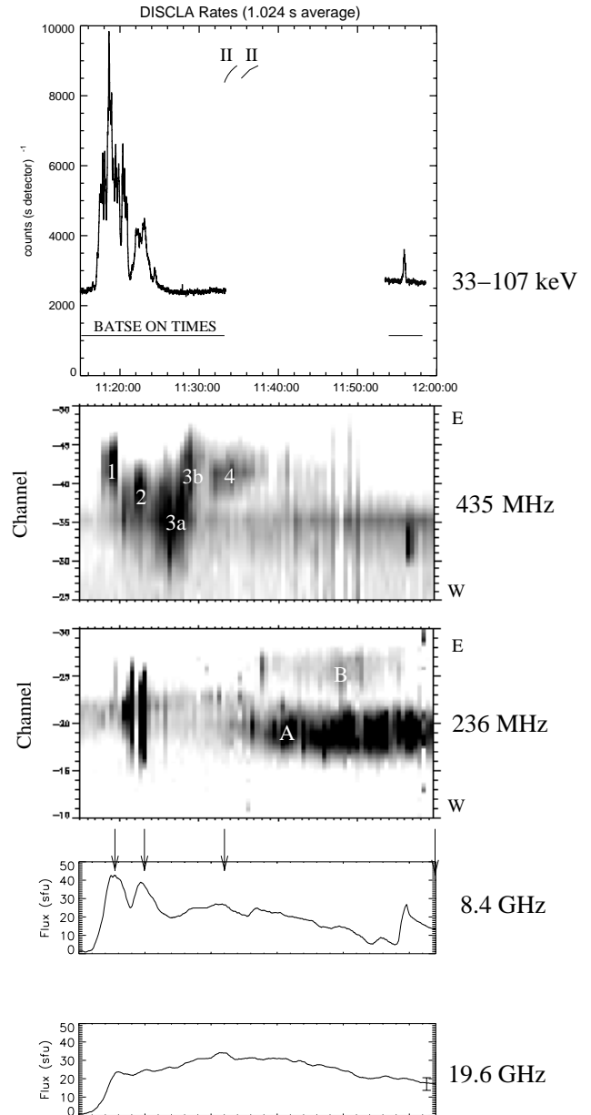
Fig. 1. Hard X-ray and radio data from June 27, 1993 at 11:15–12:00 UT. BATSE count rates in the 33–107 keV energy range (top), Nancay Radioheliograph East-West scans over the solar disk at 435 and 236 MHz (middle), and Bern full disk flux at 8.4 and 19.6 GHz (bottom). The times of the strongest type II emissions are depicted in the plot at the top. The 2-D source positions of the 1-D temporal features 1, 2, 3, and 4 (at 435 MHz), and of A and B (at 236 MHz) are given in Fig. 3. Arrows mark the times of the spectral plots in Fig. 7. The error bar in the 19.6 GHz plot marks the maximum error in flux density at that frequency around 12 UT. The error is less at earlier times and at lower frequencies.
