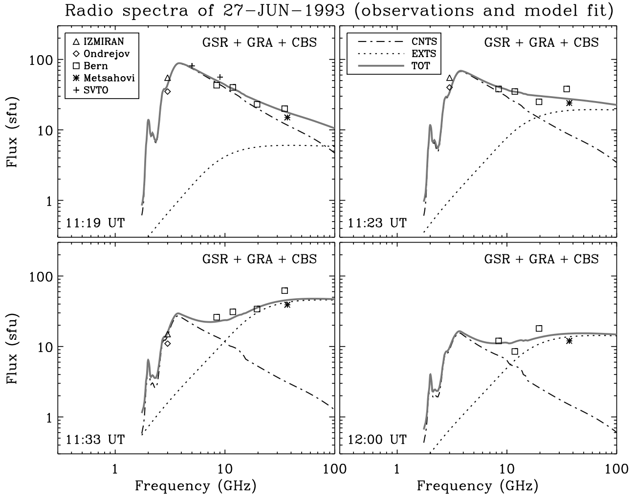
Fig. 7. Observed radio spectra at 11:19 UT, 11:23 UT, 11:33 UT, and 12:00 UT (symbols) and the relevant fits by our model calculations (lines). The solar fluxes are from different stations as given in the legend (top left). The Ondřejov, Bern, and Metsähovi radio fluxes are calculated relative to the quiet Sun level. The top-right legend explains the calculated fluxes: thin black lines show the contributions of the two different sources (CNTS – compact nonthermal source, EXTS – extended thermal source; see Table 2 and Figs. 5, 6). Thick gray lines refer to the resultant spectra. All flux values are corrected to the quiet Sun level. Further explanations are given in the text.
