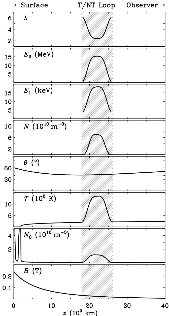
Fig. 5. Height profiles of the parameters in the compact nonthermal source (CNTS) used for the model calculations in order to interpret the observed spectrum at 11:33 UT. The hatched range marks the loop with thickness L = 8000 km located at z = 22000 km where temperature and density of the background plasma are enhanced. Only inside the loop nonthermal (power-law) electrons are assumed (top four panels). All parameters show a smooth behaviour, i.e., the most extreme (energetic) values occur around the center decreasing in direction to the loop boundary (no “jumps”).
