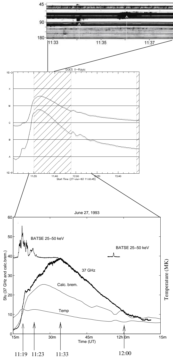
Fig. 2. From top to bottom: IZMIRAN dynamic spectra at 45–180 MHz at 11:33–11:38 UT on June 27, 1993. Arrows mark the strongest fragmented type II radio emission features in the plot. The times of the strongest type II features are also marked in Fig. 1. GOES soft X-rays on June 27, 1993 during 11:00–13:00 UT, where the shaded areas represents Yohkoh satellite night time. Metsähovi 37 GHz flux from the active region area (2.4 arcmin beam area) during 11:15–12:15 UT. The “calc. brem.” curve shows the calculated amount of thermal bremsstrahlung at the same frequency, and “temp” the calculated plasma temperature (from GOES soft X-ray flux, assuming isothermal plasma density). Arrows mark the times of the spectral plots in Fig. 7.
