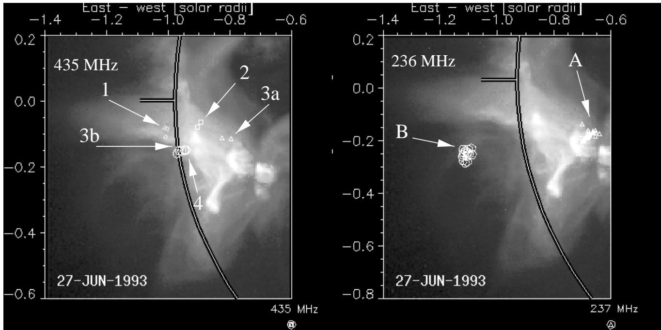
Fig. 3. Left: Yohkoh SXT soft X-ray image at 12:40 UT (post-flare), with radio source locations 1, 2, 3a, 3b, and 4 at 435 MHz. Right: radio source locations A and B at 236 MHz over the Yohkoh image. The source locations correspond to the burst features seen in the spectra, presented in Fig. 1.
