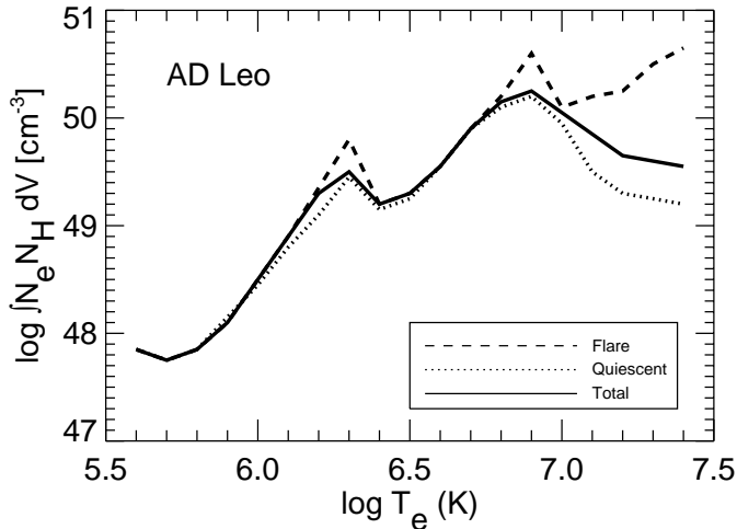
Fig. 5. Emission measure ( \log \int N_e N_H dV ( \text{cm}^{-3} )) as a function of \log T_e (K) for AD Leo during summed (solid line), flaring (dashed line) and quiescent (dotted line) stages. The EMD above \log T_e(K) = 7.4 is uncertain (see text).
