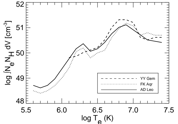
Fig. 6. Emission measure ( \log \int N_e N_H dV ( \text{cm}^{-3} )) as a function of \log T_e (K) for AD Leo (dM3e), FK Aqr (dM2e/dM3e) and YY Gem (dM1e/dM1e), weighted by their stellar radii in solar units. EMD of FK Aqr and YY Gem was taken from Sanz-Forcada et al. (2002a).
