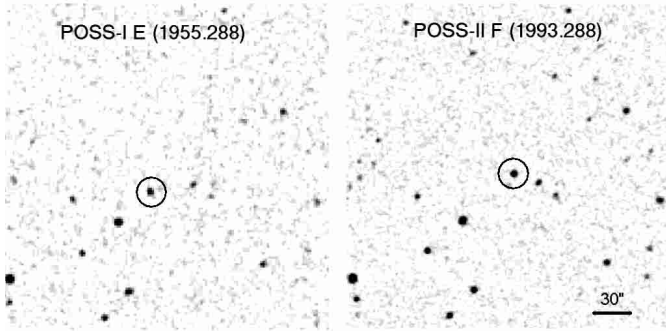
Fig. 1. First epoch (POSS-I, XE322) and second epoch (POSS-II, XP443) plates in the direction of the newly discovered WD, the encircled star near the field center. The large relative motion of the object is evident.
