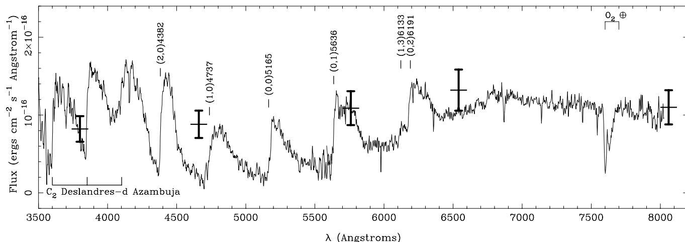
Fig. 2. The WHT optical spectrum of GSC2U J131147.2+292348. Vertical marks indicate the locations of the strong C_2 Deslandres-d'Azambuja and Swan bands, and of the telluric O_2 . The crosses refer to the fluxes (with \pm 20\% error bars) derived from the B_J , V_{12} , R_F , I_N photographic photometry of Table 2 and the U mag from Moreau & Reboul (1995).
