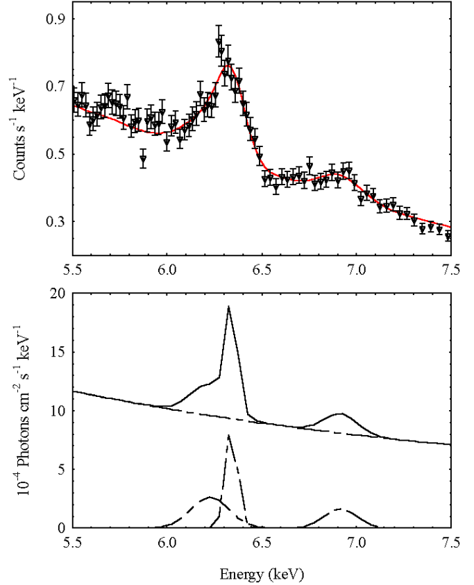
Fig. 5. Fit to the iron emission lines in the PN spectrum (left, lines 1 and 2 (Fe K\alpha ); right, line 3). Top panel: data (black) and model (red). Bottom panel: overall model (solid line) and model components (dotted line).
