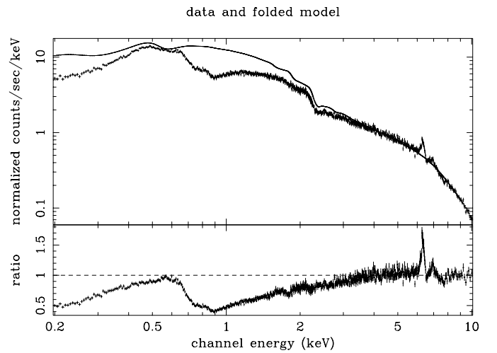
Fig. 4. Continuum power-law fit to the 3.5–5.5 and 7.5–10 keV ranges of the PN spectrum, extrapolated over 0.2–10 keV. The ratio of the data to the continuum model is shown in the bottom panel.
