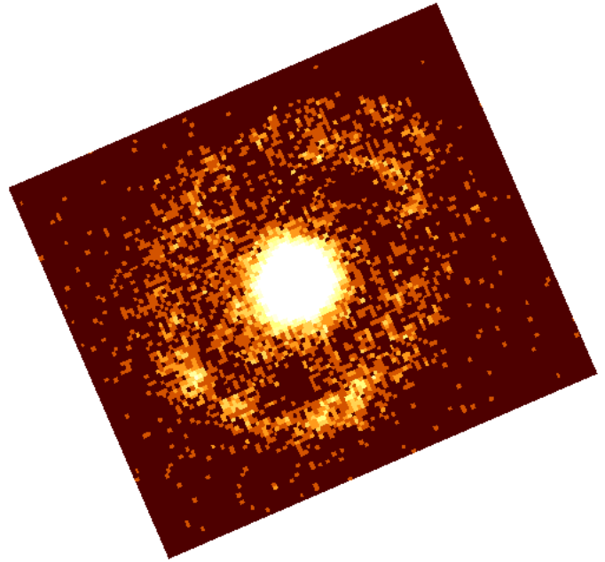
Fig. 1. UV image of NGC 3783; North is up, East to the left, and the image is about 50×40'' in size. The nuclear image is saturated in order to show the spiral arms. (This figure is available in color in electronic form.)
