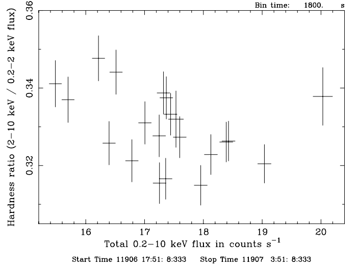
Fig. 3. Hardness – intensity plot in 30 min time bins.
