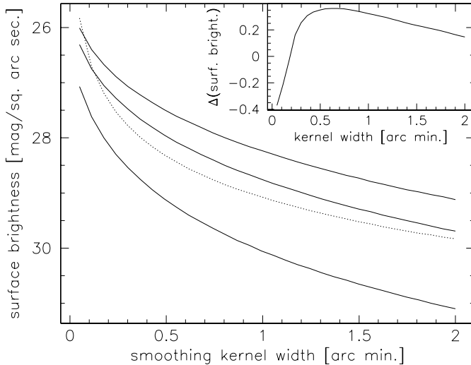
Fig. 5. Central surface brightness in the r' band (in magnitudes per square arcsec) as a function of smoothing radius for clusters of masses M = (10^{14}, 3 \times 10^{14}, 10^{15}) M_{\odot}/h at redshift z = 0.75 (solid curves from bottom to top), and the 5\text{-}\sigma sky brightness fluctuations (dotted curve). The small panel shows the difference between the solid curve for M = 3 \times 10^{14} M_{\odot}/h and the dotted curve, i.e. the signal-to-noise ratio as a function of the smoothing radius. It has a broad peak at \Delta\theta \sim 0.5' .
