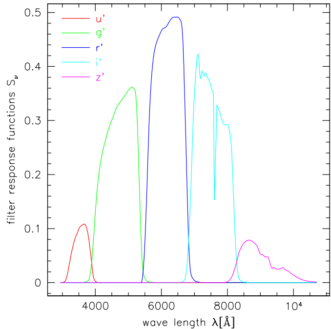
Fig. 1. Recently re-measured SDSS filter response functions. From left to right: u' , g' , r' , i' , and z' .
