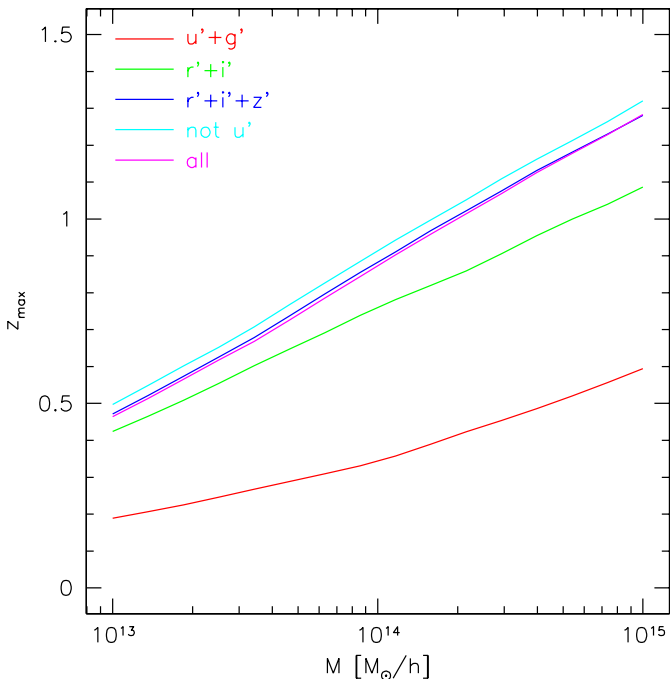
Fig. 8. 5\text{-}\sigma detection limits for clusters as a function of mass in several combinations of wave bands. Solid curve: ( u' + g' ); dotted curve: ( r' + i' ); short-dashed curve: ( r' + i' + z' ); long-dashed curve: all bands except u' ; dash-dotted curve: all bands.
