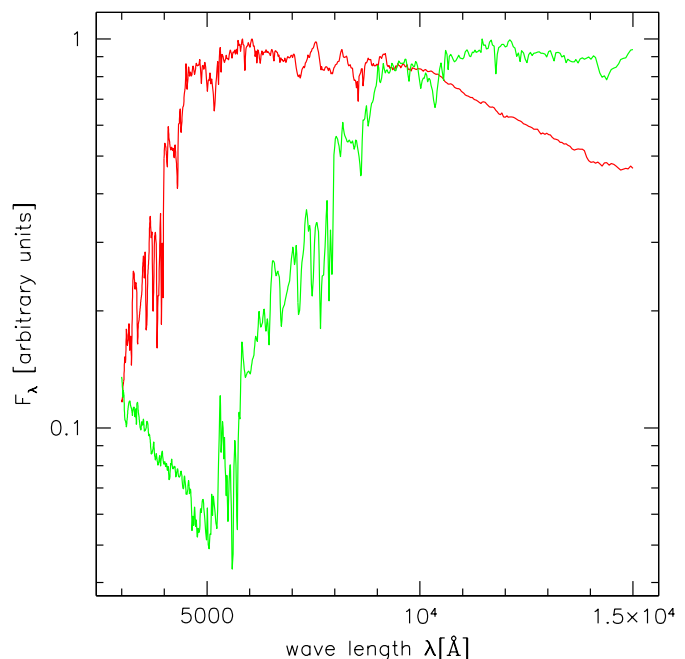
Fig. 2. Composite cluster spectra F_{\lambda}^C as functions of wavelength \lambda in \text{\AA} , at redshifts zero (solid curve) and unity (dotted curve). Both spectra are arbitrarily normalised.
