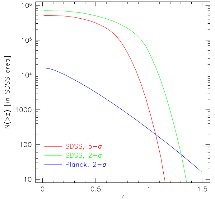
Fig. 10. Cumulative redshift distributions N(>z) of clusters with M \geq 5 \times 10^{13} h^{-1} M_{\odot} in summed r'+i'+z' SDSS data, detected at 2- \sigma and 5- \sigma significance as indicated in the plot. Also shown is the cumulative redshift distribution of clusters detected through the thermal Sunyaev-Zel'dovich effect at 2- \sigma significance by the Planck satellite. Shown is the expected number of clusters in the SDSS area. The abundance of SDSS clusters lies almost two orders of magnitude above that for Planck clusters up to the redshift where clusters with M = 5 \times 10^{13} h^{-1} M_{\odot} drop below the detection limit. The SDSS abundances then cut off exponentially. All Planck clusters in the survey area are detected by SDSS out to z \sim 1.1 at 5- \sigma , and out to z \sim 1.3 at 2- \sigma . Cluster catalogues constructed from the SDSS data by more traditional techniques are expected to be complete out to redshift z \sim 0.4 (Kim et al. 2001), and so should contain about 20% of the clusters in these deeper catalogues.
