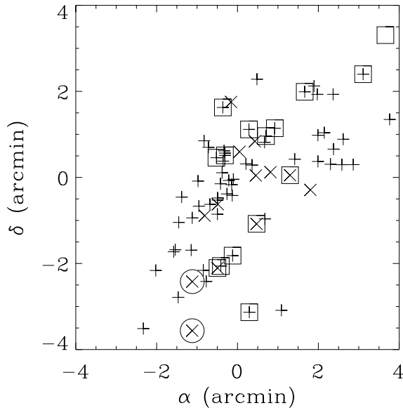
Fig. 8. Spatial distributions of early-type galaxies (crosses), late-type galaxies (X's), galaxies with EW(H\delta) \geq 3 \text{ \AA} (squares) and galaxies with emission lines (circles). Only galaxies with velocities in the cluster velocity range are shown.
