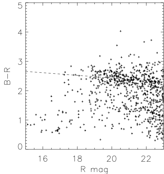
Fig. 1. B-R vs. R distribution of the galaxies within the cluster field. The dashed line is a fit to the points with 17 < R < 21.5 and 2.1 < B-R < 2.8 , B-R = 3.33 - 0.045 R , and defines the CM sequence of the early-type population of cluster members.
