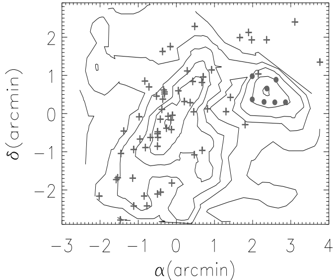
Fig. 2. 2D projected density of (likely) cluster members, selected within \pm 0.5 mag of the B - R vs. R CM sequence. The 2D-density is estimated using the Adaptive Kernel Method. The three highest-density contours correspond to 9, 12 and 24\sigma levels. North is up, East is to the left. Crosses indicate galaxies with measured velocities that belong to the main cluster, dots indicate galaxies with measured velocities that belong to a subcluster, according to the KMM algorithm partition (see text).
