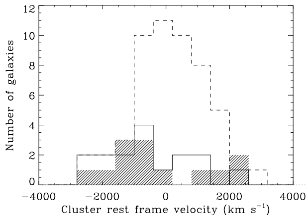
Fig. 9. Velocity distributions of early-type galaxies (dashed line), late-type galaxies (shaded histogram), galaxies with EW(H\delta) \geq 3 \text{ \AA} (solid line), in the reference frame of the cluster. Only cluster members are considered; galaxies belonging to the subcluster have been removed from the sample.
