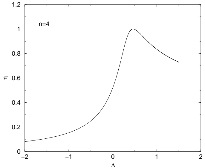
Fig. 9. Phase diagram for n = 4 .
