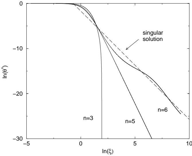
Fig. 1. Density profiles of polytropes with index n = 3, 5, 6 . The dashed line corresponds to the singular solution (9).
