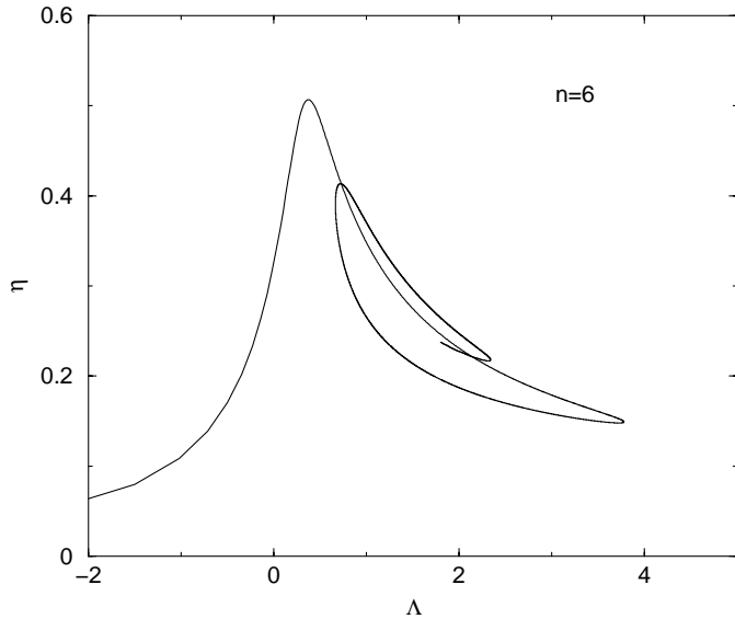
Fig. 10. Phase diagram for n = 6 .
