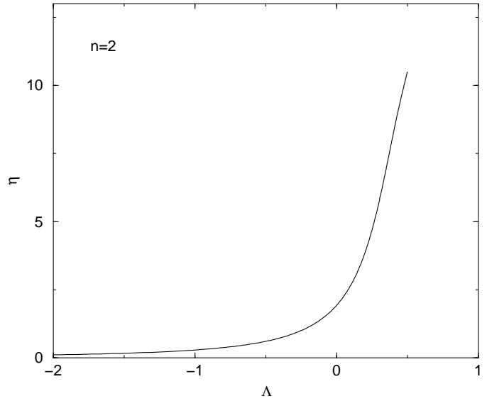
Fig. 8. Phase diagram for n = 2 .
