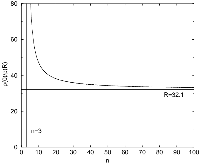
Fig. 7. Critical density contrast as a function of the polytropic index n .
