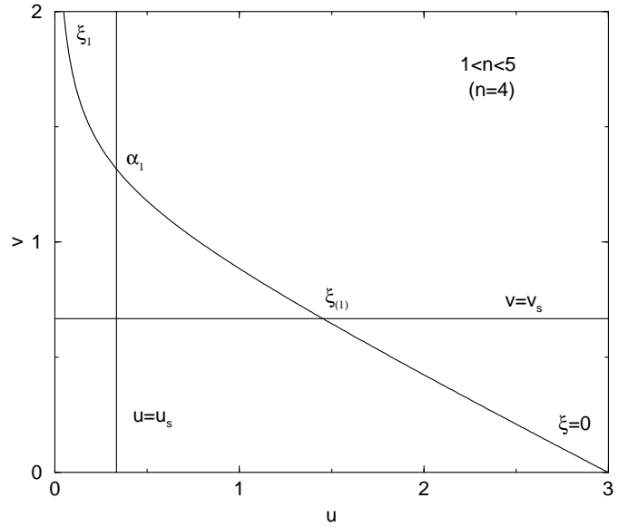
Fig. 2. The (u, v) plane for polytropes with index 1 < n < 5 . The construction is made explicitly for n = 4 .
