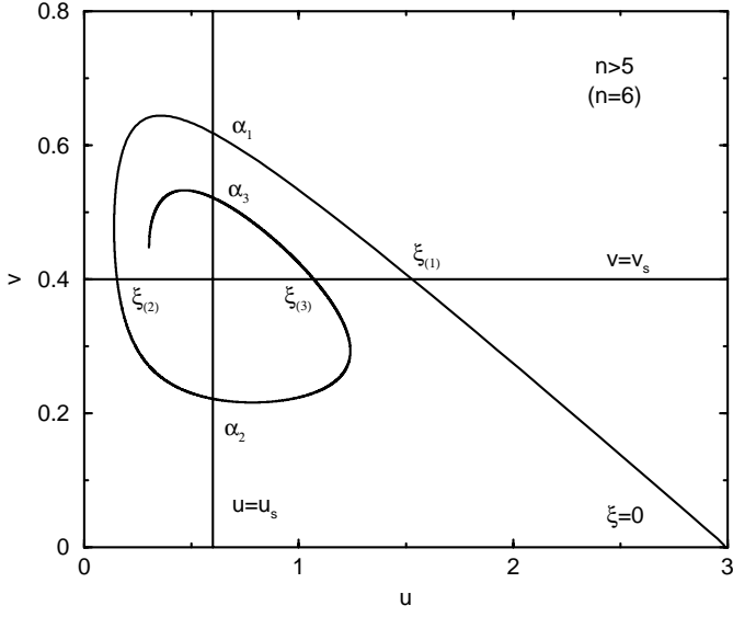
Fig. 4. The (u, v) plane for polytropes with index n > 5 . The construction is made explicitly for n = 6 .
