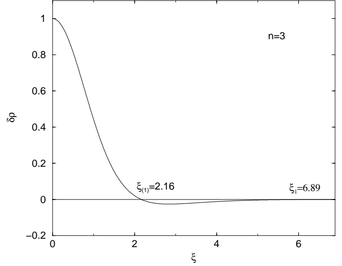
Fig. 6. Density perturbation profile for the critical polytrope of index n = 3 .
