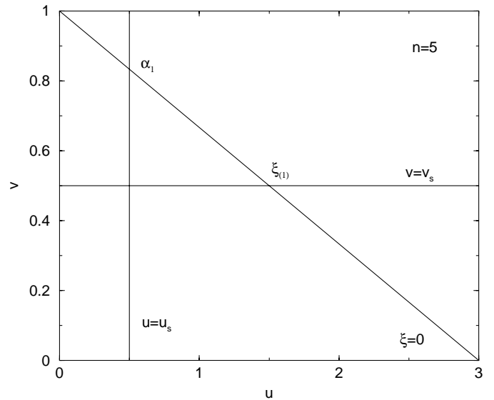
Fig. 3. The (u, v) plane for polytropes with index n = 5 .
