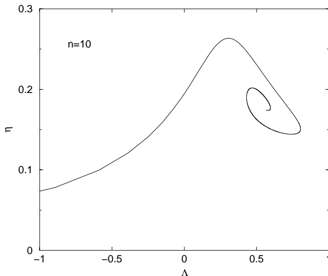
Fig. 11. Phase diagram for n = 10 .
