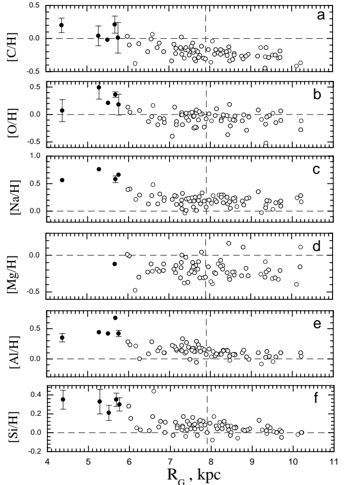
Fig. 2. Same as Fig. 1, but for elements C–Si.
