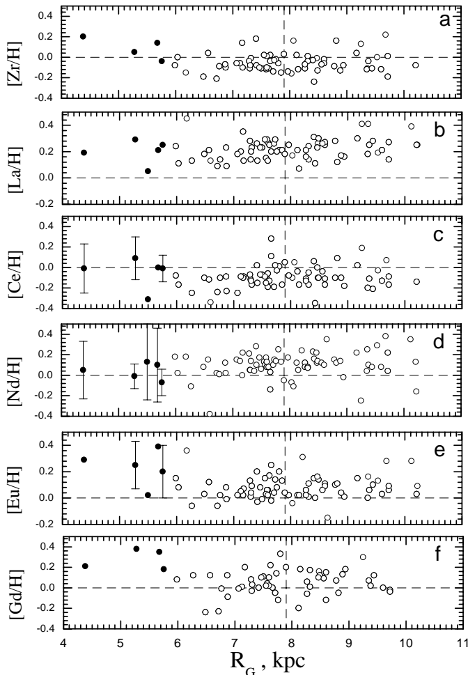
Fig. 5. Same as Fig. 1, but for elements Zr–Gd.
