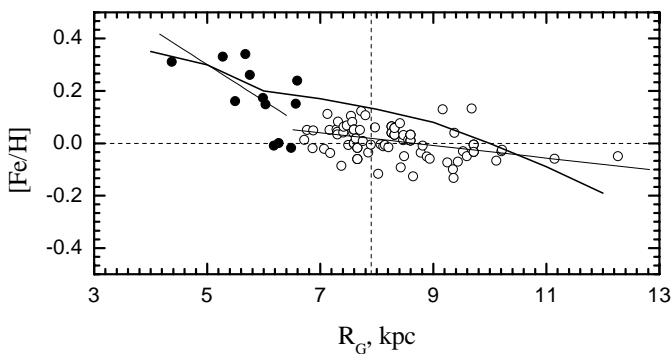
Fig. 6. The radial distribution of the iron abundance for two zones. Open circles and black circles represent the Cepheids separated at 6.6 kpc. Theoretical prediction of “inside-out” model A (Chiappini et al. 2001 – thick line ).
