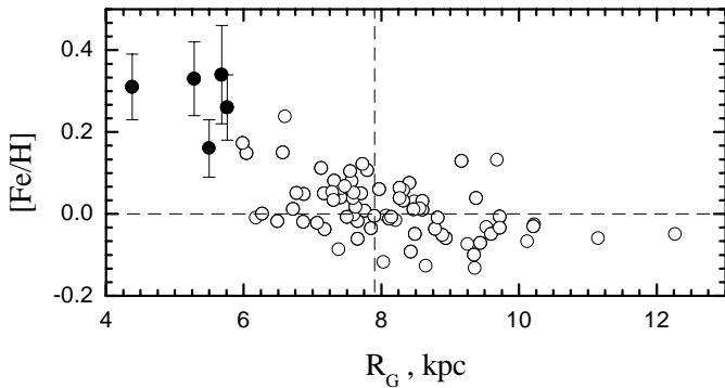
Fig. 1. The radial distribution of the iron abundance. Open circles – data from Paper I, black circles – present results. 2\text{-}\sigma interval is indicated for the stars from present study.
