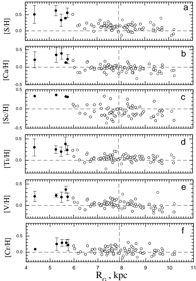
Fig. 3. Same as Fig. 1, but for elements S–Cr.
