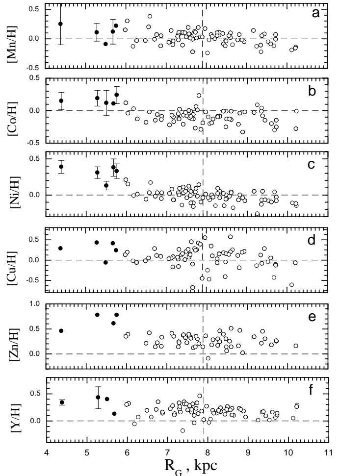
Fig. 4. Same as Fig. 1, but for elements Mn–Y.
