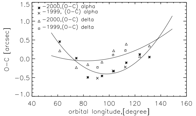
Fig. 9. Metis: dependence (O–C) on the orbital longitude of the satellite.
