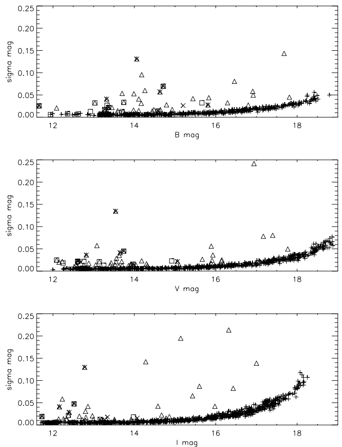
Fig. 1. Mean stellar magnitude versus rms variations in the B (top), V (middle) and I light curves of run 1. Variables are indicated with triangles, spectroscopic binaries with squares, X-ray sources with crosses. Non-variable stars are defined by the lower envelope of points.
