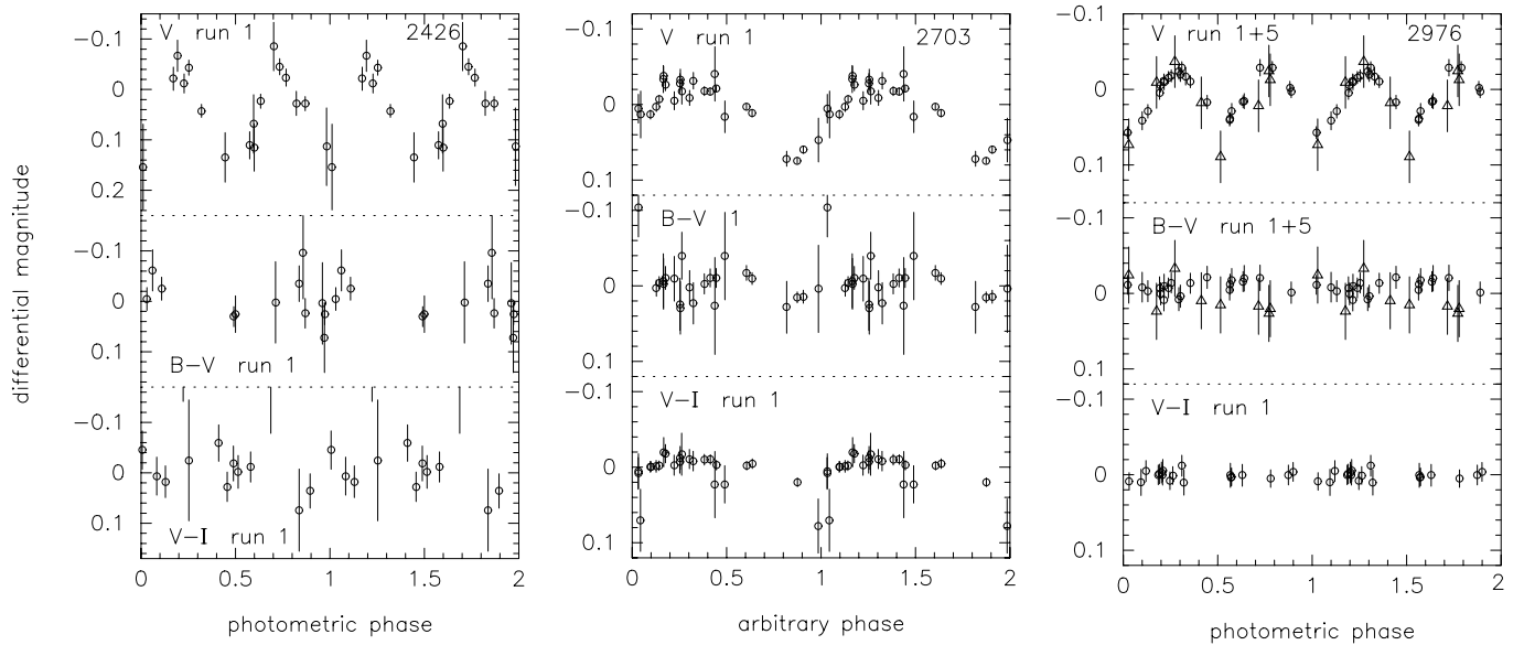
Fig. 3. Light and colour curves for stars 2426, 2703 and 2976 (S757) folded on the periods of 0.2888, 3.7 and 0.3600 days, respectively (see text, Sect. 3.3). Data from different observing runs are marked with different symbols: open circles for run 1, open triangles for run 5.
