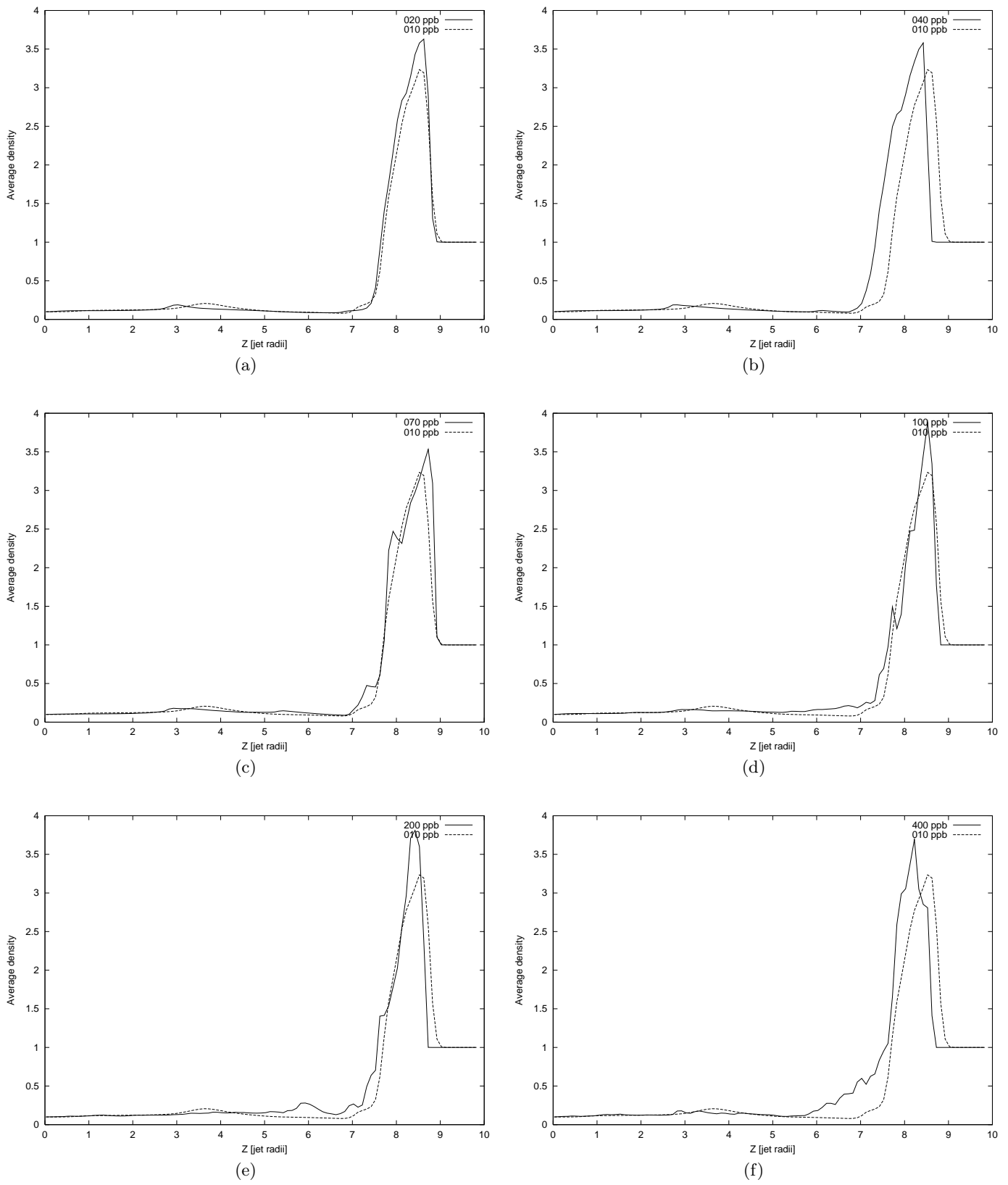
Fig. 16. Density averaged over the beam radius for the simulations of setup B. Plots a to f apply to 20 ppb, 40 ppb, 70 ppb, 100 ppb, 200 ppb and 400 ppb, respectively. The mass entrainment into the jet head can be seen in plot f, between Z = 6 and Z = 7.5 . For comparison, the 10 ppb curve is plotted as a dashed line in each figure.
