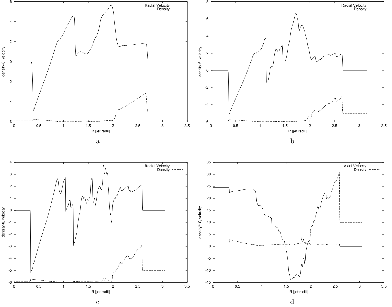
Fig. 9. a)–c): Slices at Z = 1.5 for radial velocity (solid) and density ( \cdot 6 ) (dashed) over radius at time t = 0.5 for setup B. The resolution is 100, 200, and 400 ppb for plot a) to c), respectively. The shocked external medium is located between R = 2 and R = 2.7 . d) Radial slice for density ( \cdot 10 ) and axial velocity at t = 0.5 , Z = 1.5 for the 400 ppb simulation. At R = 1.9 the fingers of the KH instabilities are visible (increase in the density). They also appear in the velocity as slower regions.
