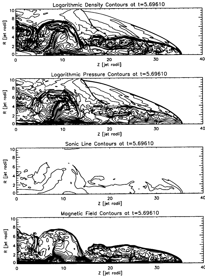
Fig. 10. Contour plots of the density (30 logarithmically spaced lines), pressure (30 logarithmically spaced lines), magneto-sonic lines (magneto-sonic Mach number equals 1 or -1 ) and toroidal magnetic field (30 lines) of the highly magnetized jet model at timestep 13 500. This corresponds to a simulation time of 5.70. In units of LPMB89 that would be 85.5.
