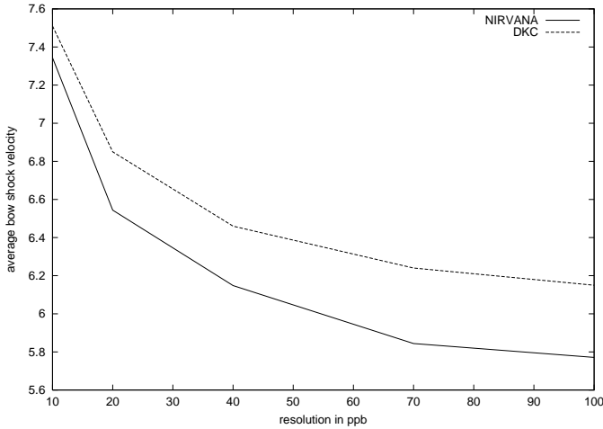
Fig. 12. Comparison of the bow shock velocity of the setup B jets with the ones of equal snapshot time from KM88. The snapshot times were: 10 ppb: t = 1.28 , 20 ppb: t = 1.41 , 40 ppb: t = 1.42 , 70 ppb: t = 1.99 and 100 ppb: t = 1.98 .
