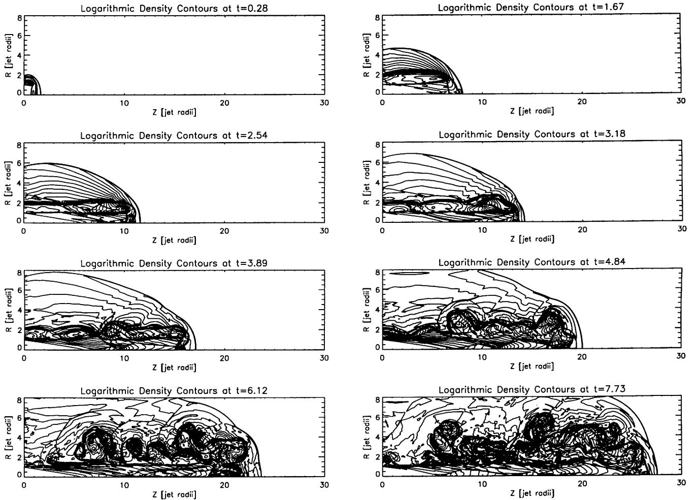
Fig. 1. Contour plots of the density (30 logarithmically spaced lines) for the jet model of setup A. The times for the snapshots were chosen in order to match Fig. 11 of KM88 closely.
