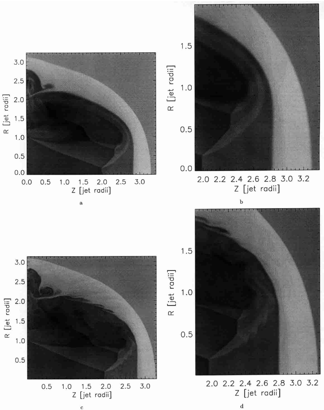
Fig. 4. Gray scale plots of the logarithmic density for the jets of setup B. On the right hand side are magnifications of the head region of the corresponding picture to the left. The upper (a) and b)) and lower (c) and d)) pictures show the 100 ppb and 200 ppb simulations, respectively. The time is 0.500 in all cases.
