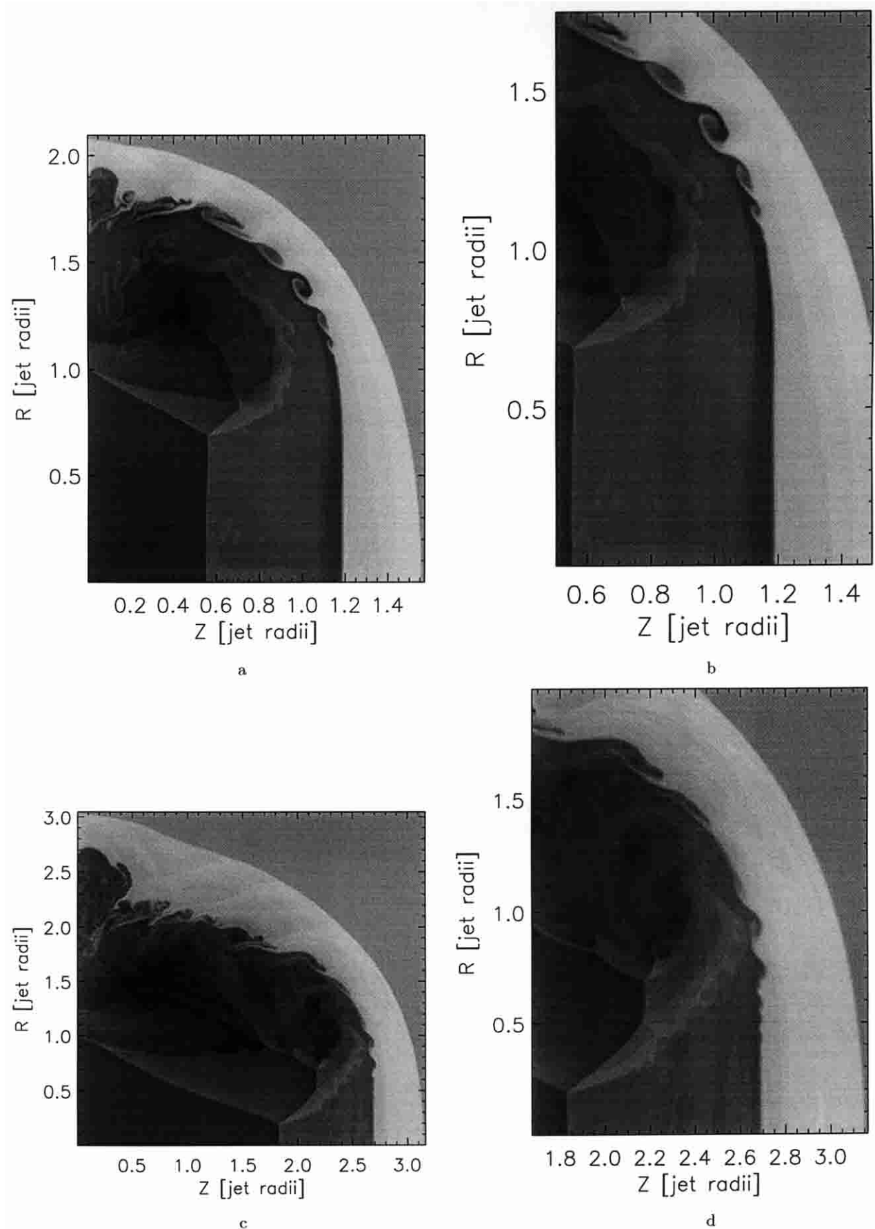
Fig. 8. Same as 4 but for 400 ppb and at times t = 0.216 (upper pictures) and t = 0.483 (lower pictures). (The data in this figure and in Fig. 4 was rebinned to 100 ppb for visualization.)
