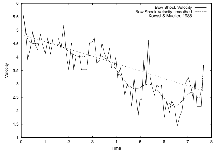
Fig. 5. Bow shock velocity over time for the jet of setup A (solid line), smoothed (long dashed line) and for comparison the approximate behavior in KM88 adopted from their Fig. 9a (short dashed line). 76 time steps were used for this graph.
