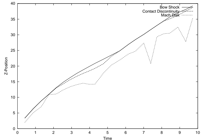
Fig. 6. Flow parameters for the hydrodynamic jet model of setup C at 15 ppb with shock handling by artificial viscosity. The vertical axis displays the z -coordinate and the horizontal axis the time in our units which is 1/15 of Lind's time unit. The highest z -value has always the bow shock, the contact discontinuity has a lower or equal z -value and the Mach disk takes the lowest value.
