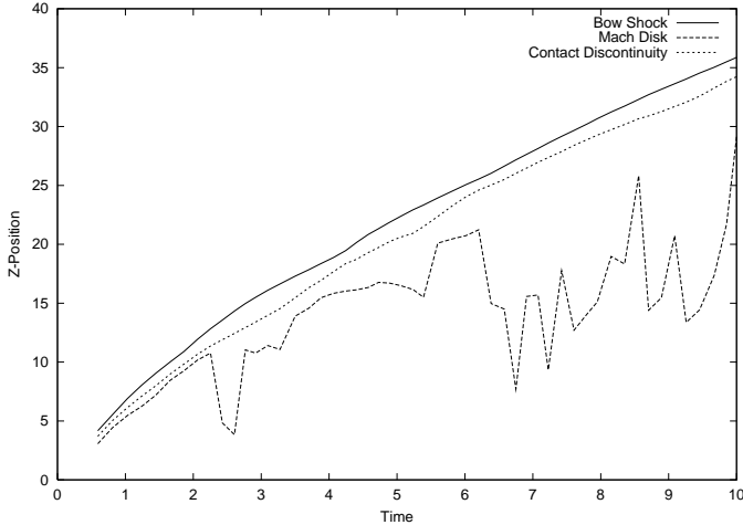
Fig. 7. Same as Fig. 6, but at a higher resolution of 30 ppb.
