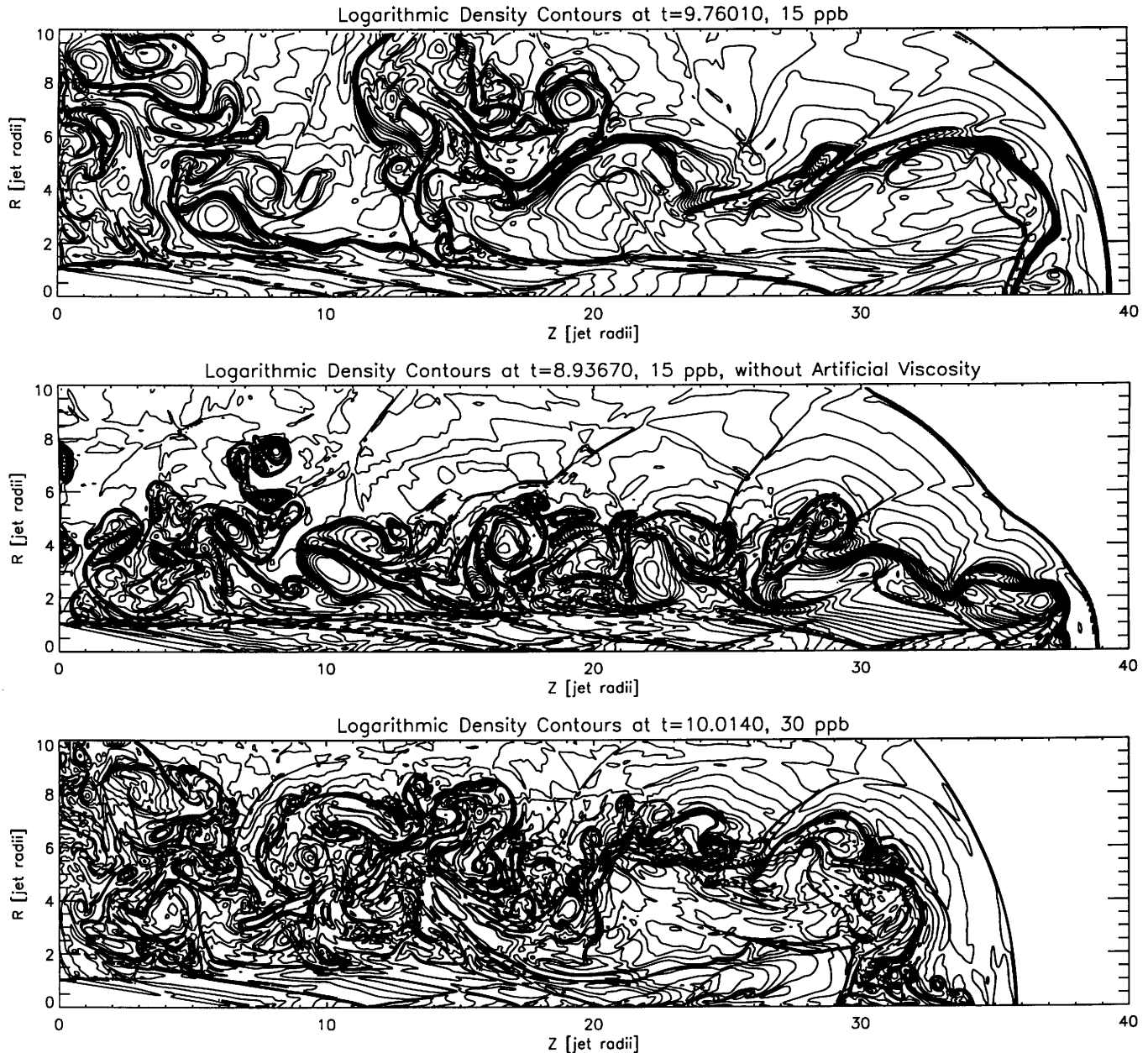
Fig. 2. Logarithmic density plot of the jet from setup C. Top: 15 ppb resolution, t = 9.76 ; middle: 15 ppb resolution without artificial viscosity, t = 8.94 ; bottom: 30 ppb resolution, t = 10.01 .
